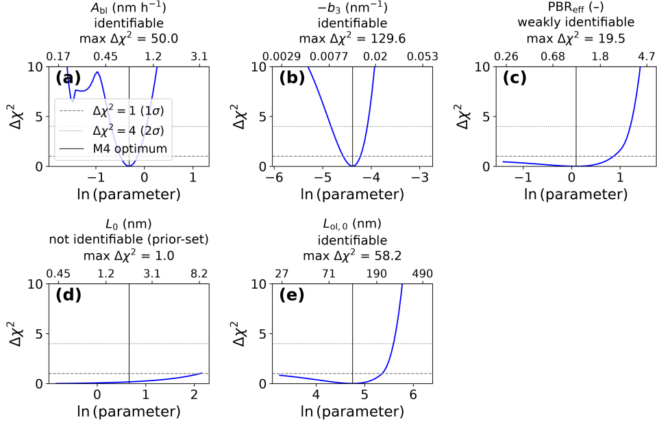
Fig. 3 Profile-likelihood identifiability map: \Delta\chi^2 over the data residuals versus each M4 parameter, with the 1\sigma ( \Delta\chi^2 = 1 ) and 2\sigma ( \Delta\chi^2 = 4 ) thresholds marked. Panels are the five M4 parameters in the order of Table 4: (a) A_{bl} , (b) -b_3 (the magnitude is plotted, b_3 itself being negative throughout), (c) PBR_{eff} , (d) L_0 , (e) L_{ol,0} . In every panel the blue curve is the profile, obtained by fixing the named parameter at each grid value and re-optimizing all the others; the vertical solid line marks the M4 optimum, and the dashed and dotted horizontal lines the two thresholds. The lower abscissa is the fitted coordinate, the natural log of the parameter magnitude; the upper abscissa is the parameter itself, in the units given in the panel title. Each panel title also carries the resulting verdict and the maximum \Delta\chi^2 attained over the scanned range: a profile that stays flat is the signature of a parameter the data do not determine. The secondary structure at low A_{bl} in (a) is re-optimization of the remaining parameters along a shallow direction; it lies far above both thresholds and does not affect the interval.
