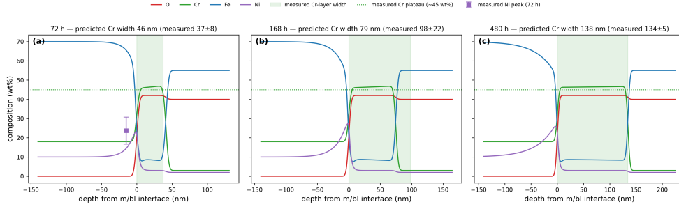
Fig. 4 Zero-free-parameter composition-map prediction against Veile et al.’s measured EDX features at (a) 72, (b) 168, and (c) 480 h. Curves are predicted composition profiles (O, Cr, Fe, Ni; weight percent) versus depth from the metal/barrier-layer interface; overlays mark the measured features compared: Cr-layer width (shaded band), Cr plateau level ( \sim 45 wt%, dotted), and the 72-h Ni-peak amplitude ( 23.7 \pm 7.0 wt%, error bar). Full digitized EDX traces are not available, so the comparison is feature-based.
