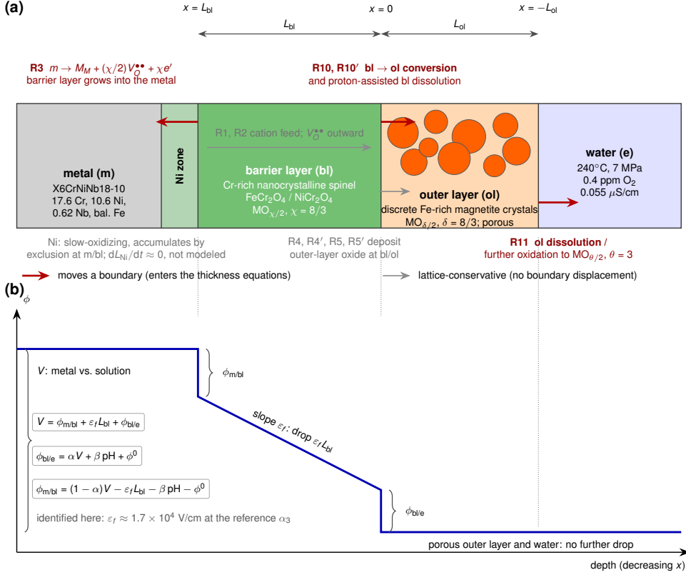
Fig. 1 Duplex-oxide model schematic, not to scale. (a) Layer structure, drawn left to right in order of increasing distance from the metal: metal | Ni enrichment zone | Cr-rich nanocrystalline spinel barrier layer | porous Fe-rich outer layer of discrete magnetite crystals | hydrothermal water. Interface positions carry the coordinate convention of the SI (Section S1.1), and the two state variables L_{bl} and L_{ol} are dimensioned above the stack. Each reaction is drawn at the interface where it acts, in red if it displaces a boundary and therefore enters Eqs. (10)–(11), in gray if it is lattice-conservative: Reaction 3 grows the barrier layer into the metal, Reactions 10 and 10' convert and dissolve it at the barrier-layer/outer-layer interface, and Reaction 11 destroys the outer layer at the outer surface. (b) Potential distribution across the same stack under the constant-field postulate. The abscissa is aligned with (a) and the ordinate is the electrostatic potential, so the decomposition V = \phi_{m/bl} + \varepsilon_f L_{bl} + \phi_{bl/e} reads off the profile directly: a step at each of the two interfaces that carries a drop, and between them the constant slope \varepsilon_f of Eq. (2). The porous outer layer carries no further drop.
