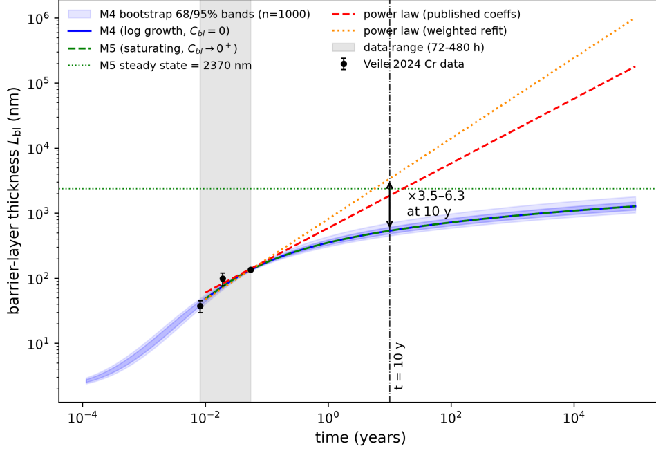
Fig. 5 Long-time prediction with propagated parametric uncertainty: M4 (blue solid, logarithmic growth) versus M5 (green dashed, saturating branch, with its steady-state thickness marked by the green dotted horizontal line) versus the two power-law variants (red dashed at the published coefficients, orange dotted for the weighted refit), to 10^5 years on log-log axes. Shaded bands are the 68% and 95% intervals of the 1000-member parametric bootstrap propagated through the M4 closed form, conditional on the M4 model structure and the reported standard errors; the M5 curve is indistinguishable from M4 at all feasible exposures. The three digitized chromium measurements are plotted as black circles and the 72–480 h calibration window is shaded gray, so the interval the extrapolations leave is visible rather than implied. The vertical line marks the ten-year horizon, and the arrow there is the separation the paper’s conclusion rests on: the two power-law variants lie a factor of 3.5 to 6.3 above the mechanistic barrier layer and outside its 95% band.
