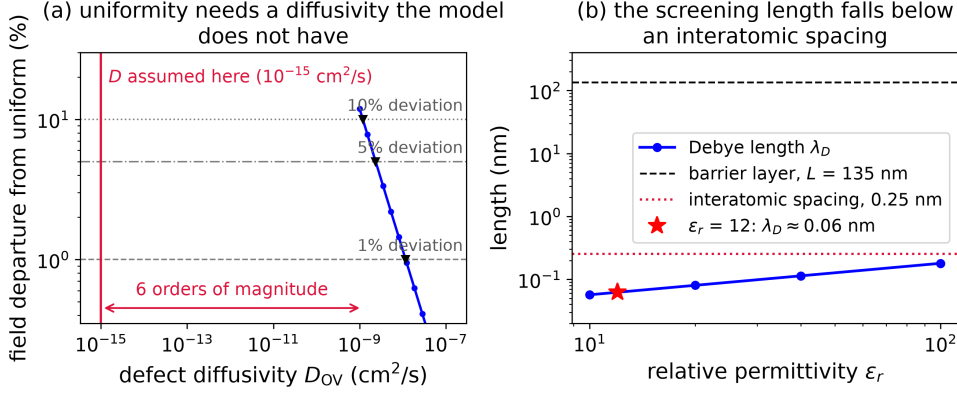
Fig. 6 The constant-field closure is not self-consistent at the transport constants the model assumes. (a) Maximum departure of the self-consistently solved field from uniform, against the oxygen-vacancy diffusivity that would be needed to hold it there; markers locate the 1%, 5% and 10% thresholds. The diffusivity actually assumed lies six orders of magnitude below all three. (b) The Debye length against its two yardsticks: the barrier layer it must screen across, and an interatomic spacing. At the permittivity used here it is approximately 0.06 nm, several times smaller than the smaller of the two, which is what makes the closure untenable rather than merely approximate.
