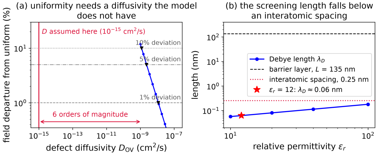
Figure 10: The constant-field closure is not self-consistent at the transport constants the model assumes. (a) Maximum departure of the self-consistently solved field from uniform, against the oxygen-vacancy diffusivity that would be needed to hold it there; markers locate the 1%, 5% and 10% thresholds. The diffusivity actually assumed lies six orders of magnitude below all three. (b) The Debye length against its two yardsticks: the barrier layer it must screen across, and an interatomic spacing. At the permittivity used here it is approximately 0.06 nm, several times smaller than the smaller of the two, which is what makes the closure untenable rather than merely approximate.
