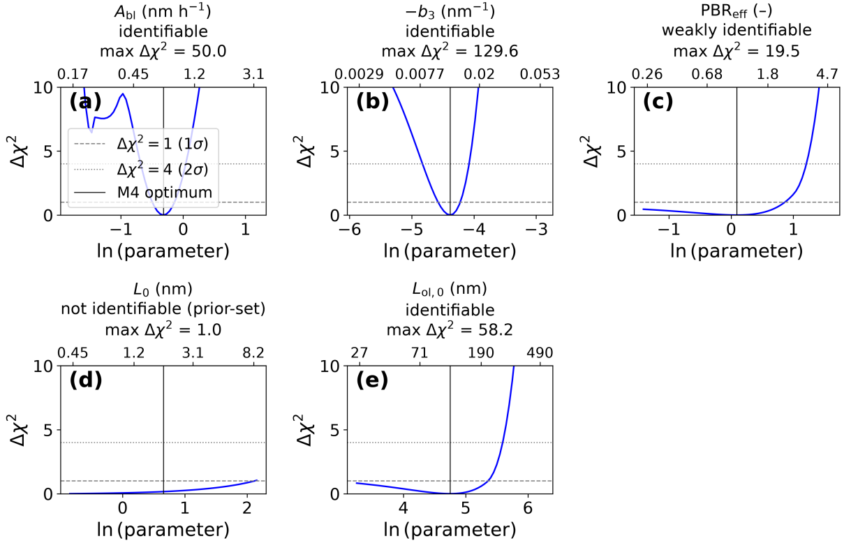
Figure 4: Profile-likelihood identifiability map: \Delta\chi^2 over the data residuals versus each M4 parameter, with the 1\sigma ( \Delta\chi^2 = 1 ) and 2\sigma ( \Delta\chi^2 = 4 ) thresholds marked. Panels are the five M4 parameters in the order of Table 5: (a) A_{bl} , (b) -b_3 (the magnitude is plotted, b_3 itself being negative throughout), (c) PBR_{eff} , (d) L_0 , (e) L_{ol,0} . In every panel the blue curve is the profile, obtained by fixing the named parameter at each grid value and re-optimizing all the others; the vertical solid line marks the M4 optimum, and the dashed and dotted horizontal lines the two thresholds. The lower abscissa is the fitted coordinate, the natural log of the parameter magnitude; the upper abscissa is the parameter itself, in the units given in the panel title. Each panel title also carries the resulting verdict and the maximum \Delta\chi^2 attained over the scanned range: a profile that stays flat is the signature of a parameter the data do not determine. The secondary structure at low A_{bl} in (a) is re-optimization of the remaining parameters along a shallow direction; it lies far above both thresholds and does not affect the interval.
