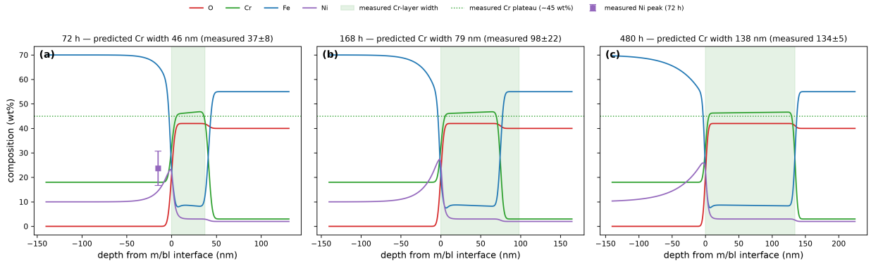
Figure 8: Zero-free-parameter composition-map prediction against Veile et al.'s measured EDX features at (a) 72, (b) 168, and (c) 480 h. Curves are predicted composition profiles (O, Cr, Fe, Ni; weight percent) versus depth from the metal/barrier-layer interface; overlays mark the measured features compared: Cr-layer width (shaded band), Cr plateau level ( \sim 45 wt%, dotted), and the 72-h Ni-peak amplitude ( 23.7 \pm 7.0 wt%, error bar). Full digitized EDX traces are not available, so the comparison is feature-based.
