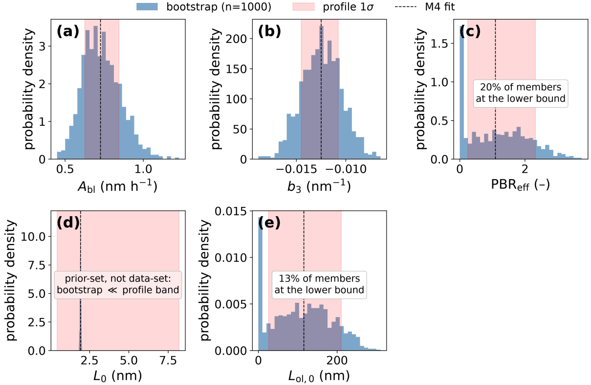
Figure 5: Bootstrap ensemble versus profile likelihood: 1000-member parametric bootstrap distribution for each M4 parameter, compared against the profile-likelihood 1\sigma band. Panels follow the order of Table 5: (a) A_{bl} , (b) b_3 , (c) PBR_{eff} , (d) L_0 , (e) L_{ol,0} . In each, the blue histogram is the distribution of the 1000 refitted values (plotted as a probability density, so panel heights are not comparable across parameters), the red shaded band is the profile-likelihood 1\sigma interval of Table 5, and the dashed vertical line is the M4 point estimate. Two annotated features are results rather than plotting artifacts. The spike at the lower bound in (c) and (e) is the fraction of resampled datasets for which the parameter is driven to zero, which is what weak identifiability looks like in a resampling ensemble. In (d) the bootstrap is far narrower than the profile band: resampling the data cannot explore a direction the data do not constrain, so the narrow histogram is not a tighter constraint but the signature of a prior-set parameter.
