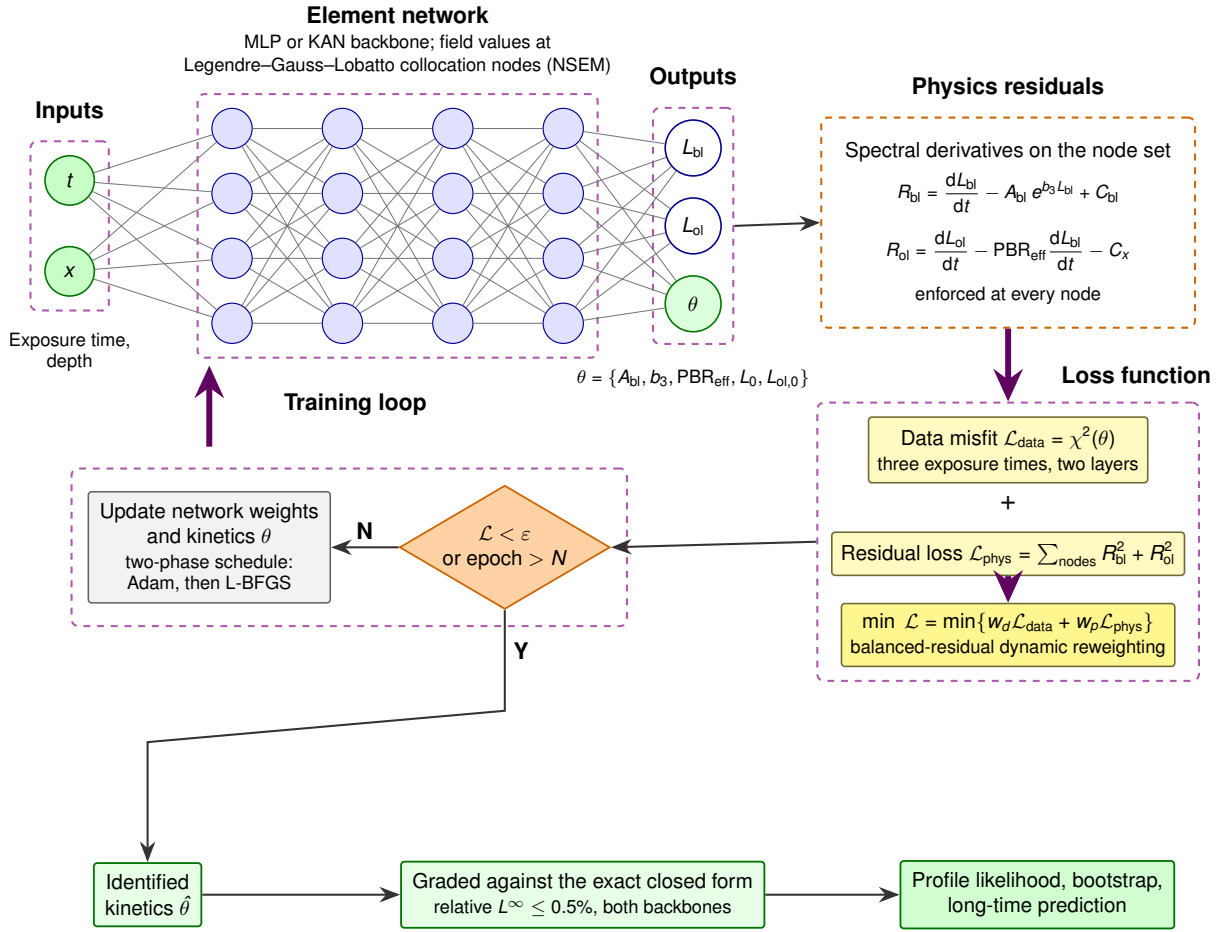
Figure 2: How the reduced model is inverted. Exposure time, and for the spatial extension depth, enters an element network whose field values are evaluated at Legendre–Gauss–Lobatto collocation nodes; the network returns the two layer thicknesses and the five kinetic parameters \theta . Spectral differentiation on the same node set gives the residuals of Eqs. (10)–(11), which are enforced at every node and combined with the data misfit of Eq. (16) by a balanced-residual dynamic reweighting of the two terms; a two-phase schedule, Adam then L-BFGS, drives the total loss to convergence. The identified kinetics are graded against the exact closed form of Eqs. (13)–(14) before they are used for profile likelihood, the bootstrap, and the long-time prediction. The solver is the neural spectral-element method (NSEM) (Tetsassi Feugmo and Pankaczy, 2026); architecture and hyperparameters for each configuration are tabulated in the SI (Section S4).
