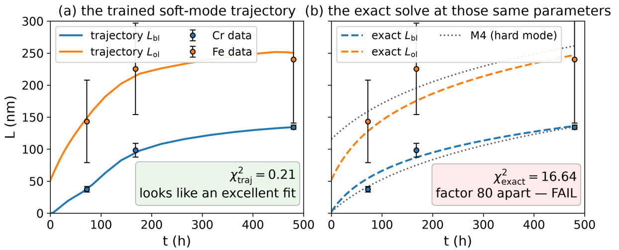
Figure 9: The F-1 failure mode. Both panels use the same six measurements and the same recovered parameters; in both, blue denotes the barrier layer and orange the outer layer, and the points are the measured means with their standard errors. (a) The trained soft-mode trajectory (solid curves), which is what the data loss sees: it passes through every point, at a \chi^2 of 0.21 that is lower than the accepted model's 5.79. (b) The exact forward solution (dashed curves) evaluated at exactly the parameters that trajectory reports, against the same data, with the hard-mode M4 solution (gray dotted) for reference: \chi^2 = 16.6 . The trajectory absorbed the misfit as slack in the governing equation, so the apparent quality of the fit in (a) is not a property of the recovered parameters. The factor of roughly 80 between the two is the diagnostic; the hard mode returns 5.79 by either route and passes by construction.
