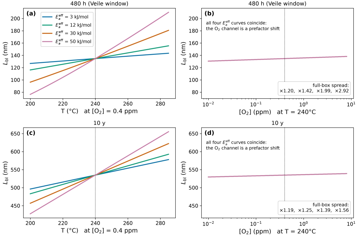
Figure 7: Operating-envelope sensitivity of the predicted barrier-layer thickness, at (a, b) 480 h and (c, d) ten years. Left panels sweep temperature at the calibration oxygen level; right panels sweep dissolved oxygen across three decades at the calibration temperature, on the same vertical scale. Each curve is one scanned value of the effective activation energy \alpha_3 \Delta G_R^0 , spanning 3–50 kJ/mol; the dotted line marks the Veile et al. calibration condition, through which every curve passes by construction. Temperature carries the sensitivity and it grows with activation energy, while three decades of dissolved oxygen shift the prediction by under six percent at 480 h and under two percent at ten years, and do so identically at every activation energy, the oxygen channel being a prefactor shift. Boxed factors are the full-envelope spreads of the four plotted activation energies, from Table 7. Contour maps over the full (T, [O_2]) box are given in the SI (Fig. S3).
