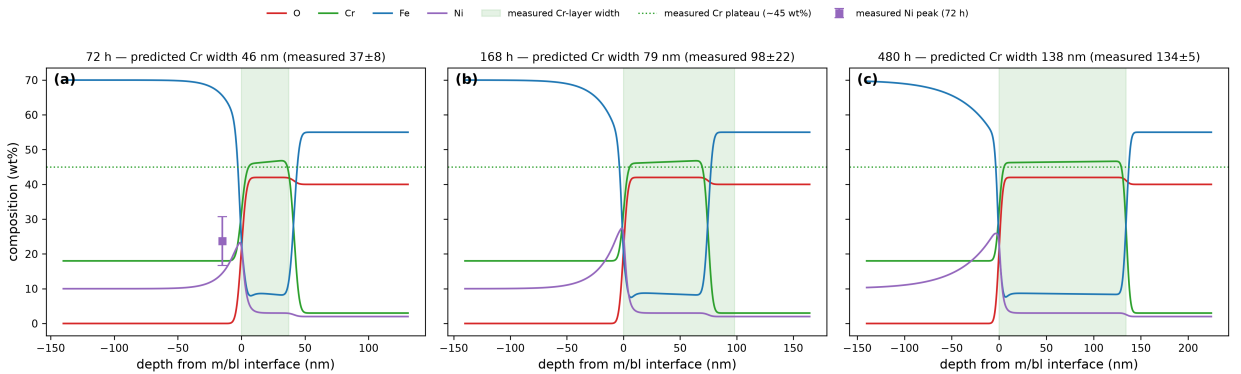
Figure 5: Zero-free-parameter composition-map prediction against Veile et al.'s measured EDX features at (a) 72, (b) 168, and (c) 480 h. Curves are predicted composition profiles (O, Cr, Fe, Ni; weight percent) versus depth from the metal/barrier-layer interface; overlays mark the measured features compared: Cr-layer width (shaded band), Cr plateau level (~45 wt%, dotted), and the 72-h Ni-peak amplitude ( 23.7 \pm 7.0 wt%, error bar). Full digitized EDX traces are not available, so the comparison is feature-based.
