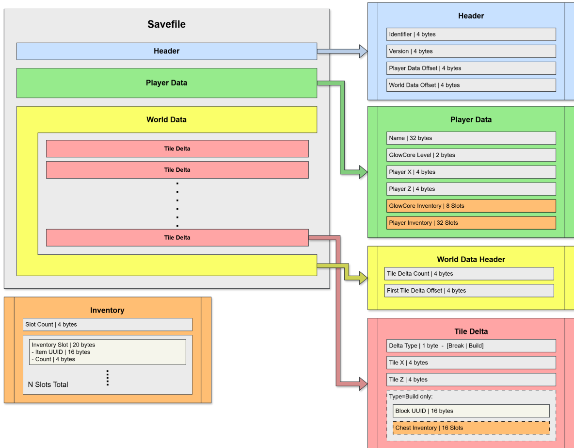
Image 14: Savefile Structure
