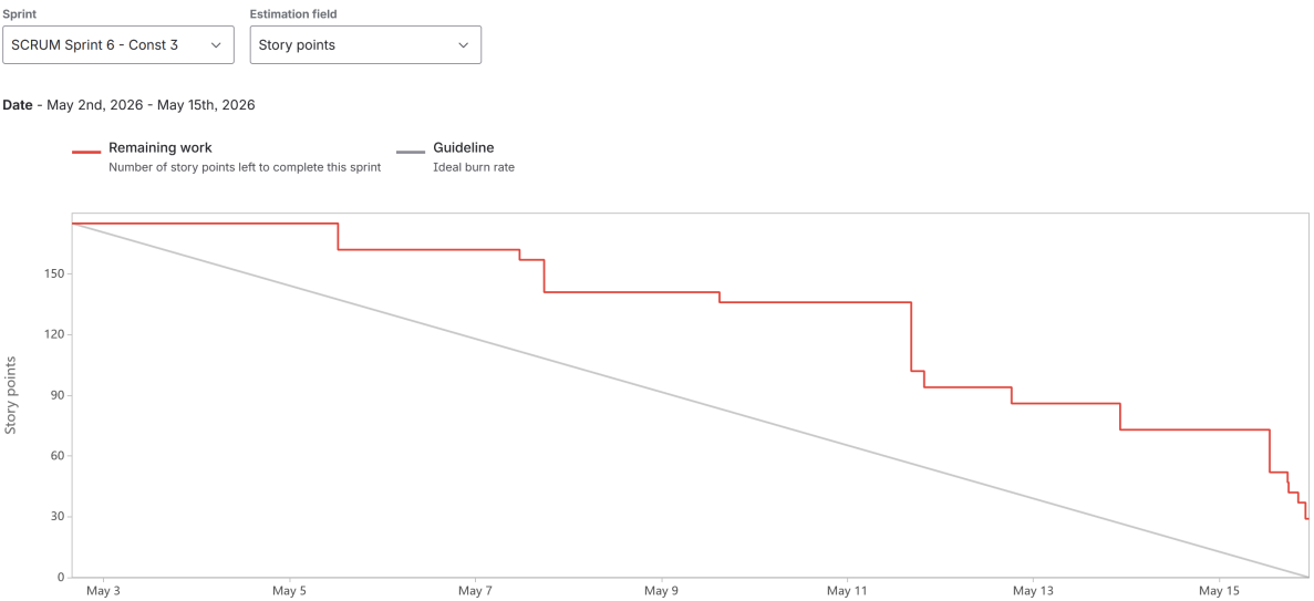
Image 41: Sprint 6 Burndown Chart
