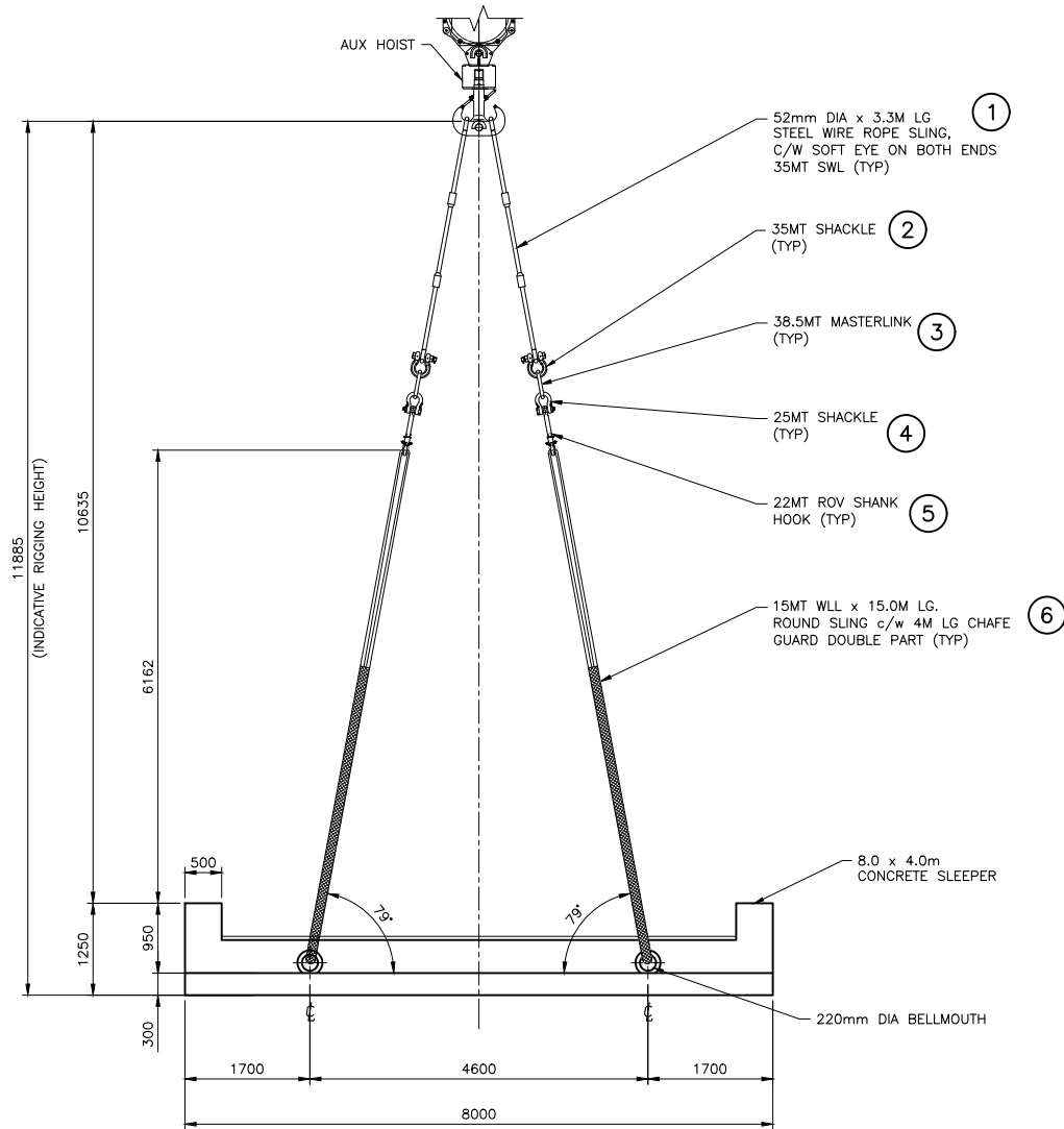
SIDE ELEVATION
