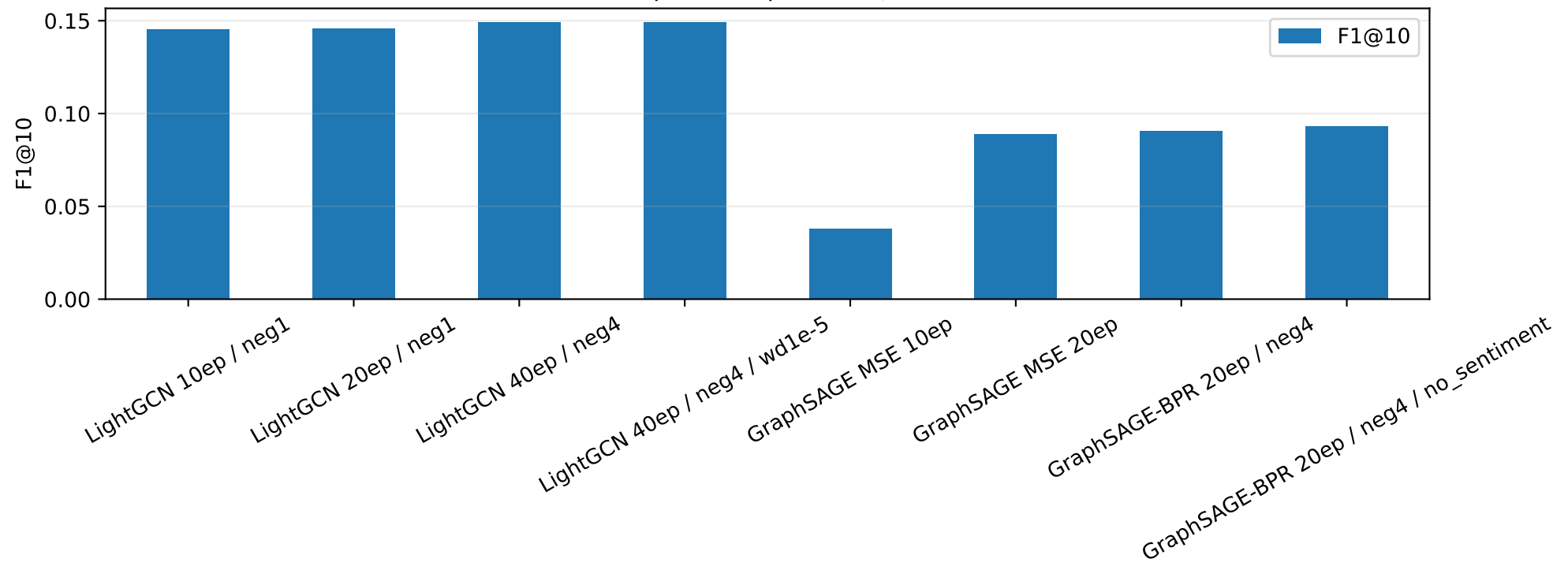
Graph checkpoint F1@10
