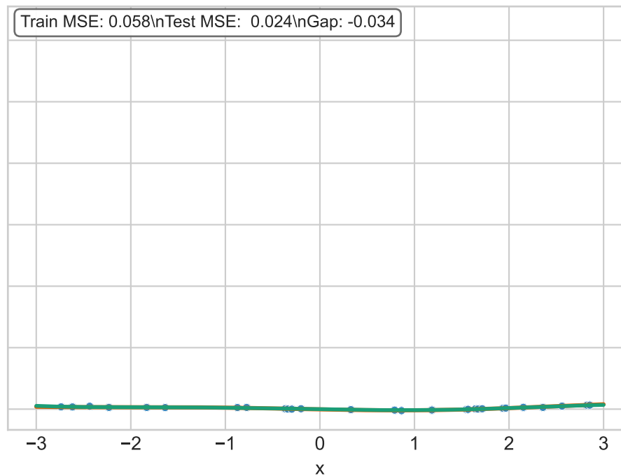
Balanced fit (degree = 5)
