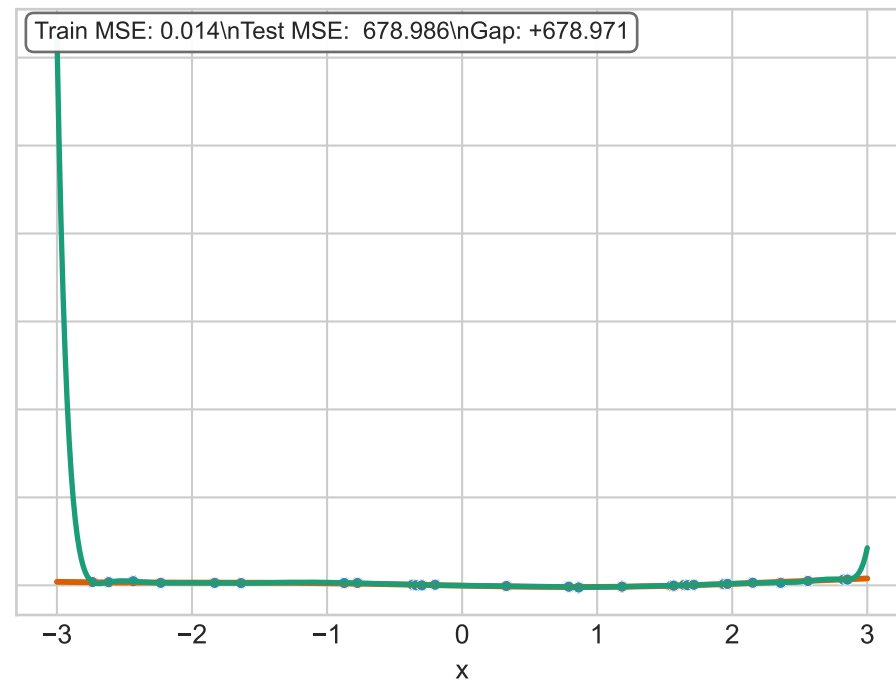
Overfitting (degree = 18)
