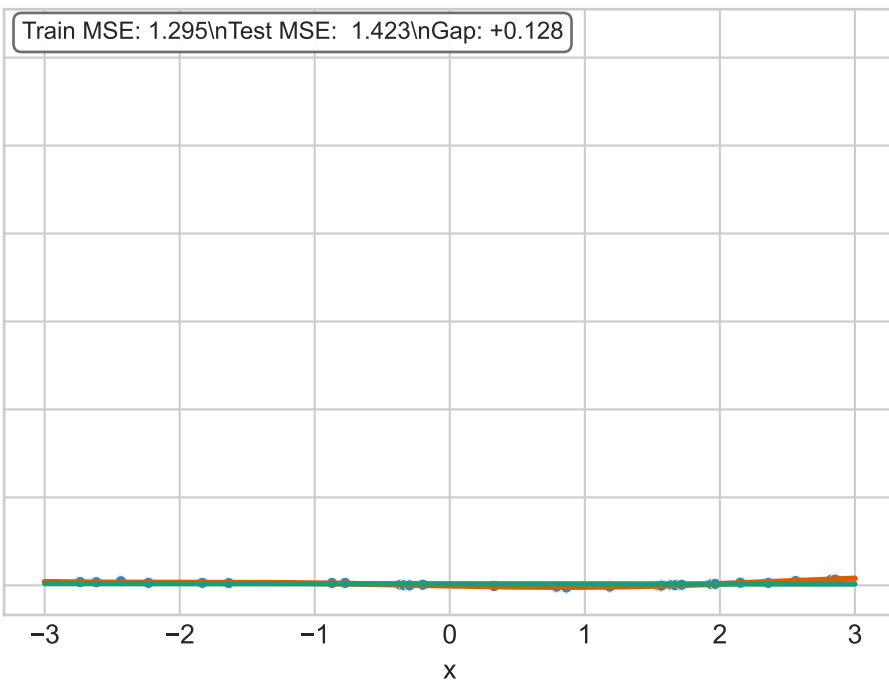
Underfitting (degree = 1)
