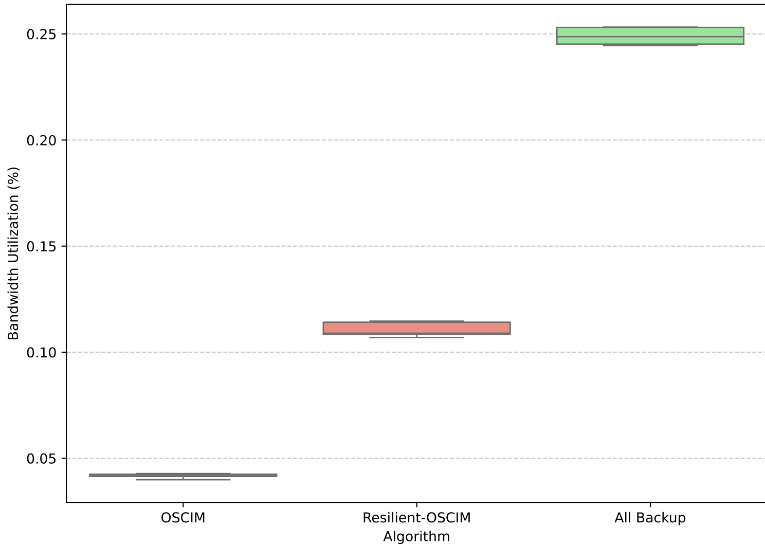
Bandwidth Utilization (%) - Boxplot
