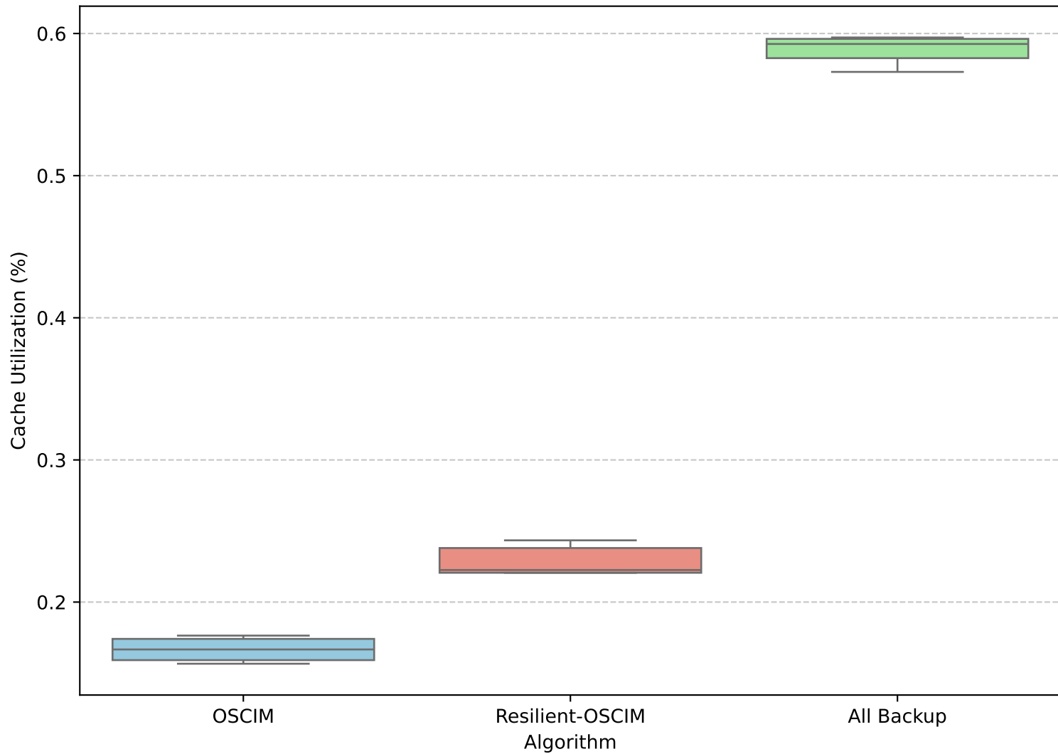
Cache Utilization (%) - Boxplot
