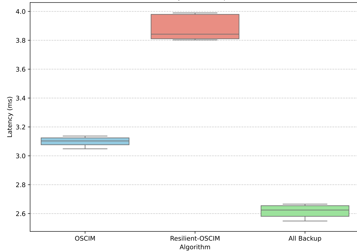
Latency (ms) - Boxplot
