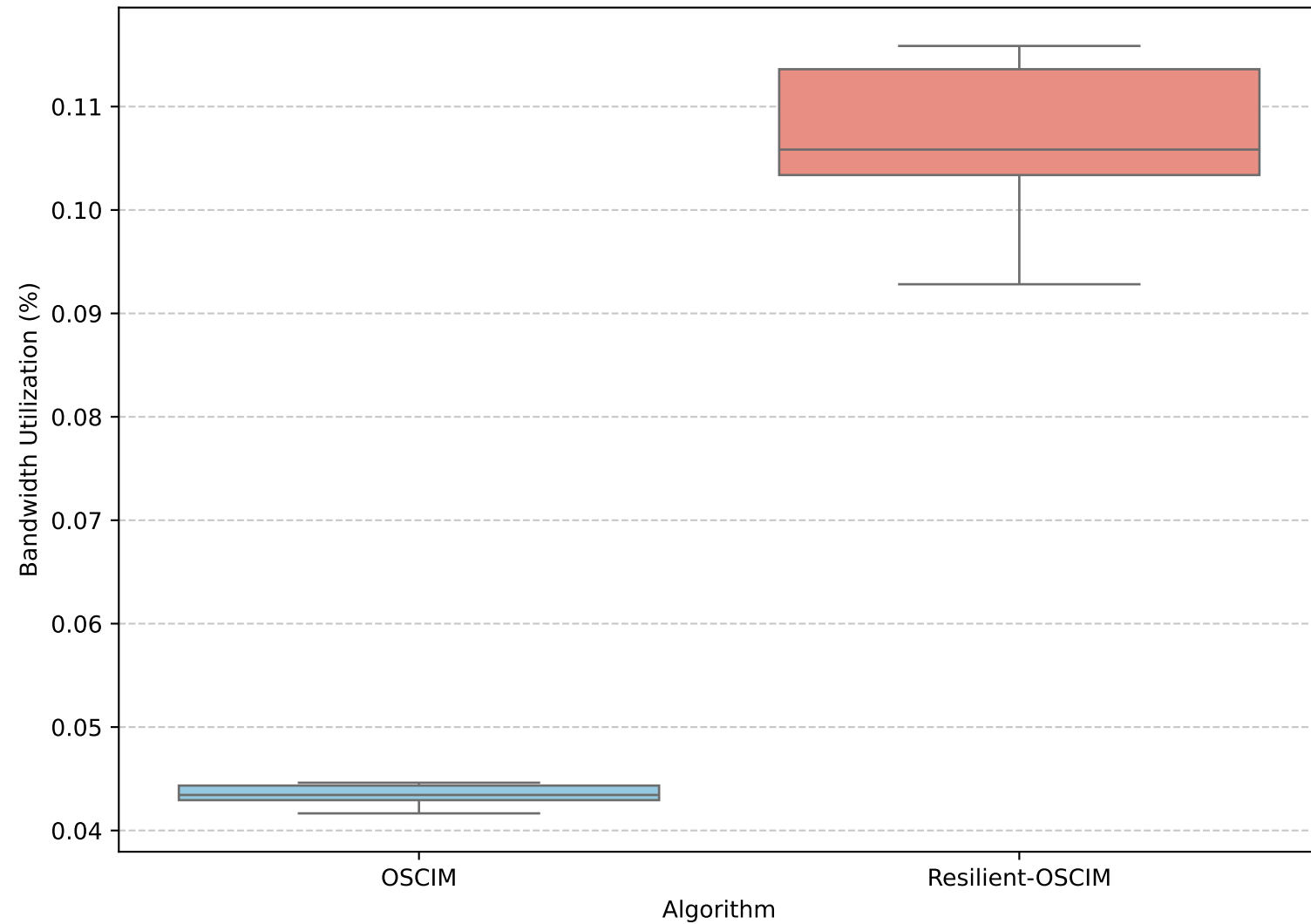
Bandwidth Utilization (%) - Boxplot
