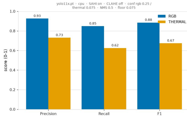
Detection scores by modality
