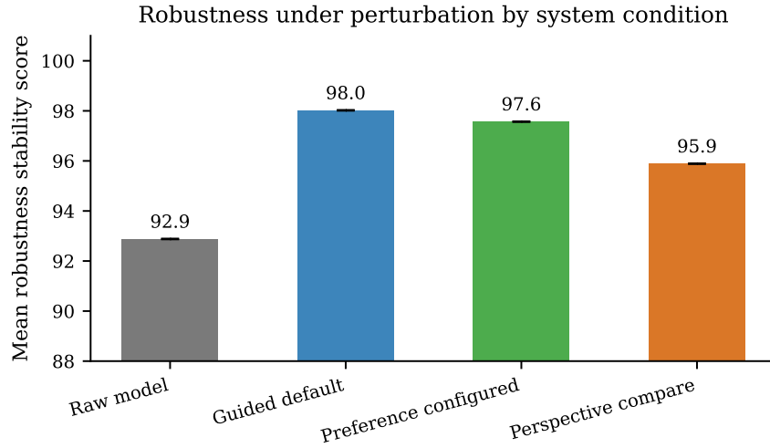
Figure 4: Stability under perturbation by system condition.
