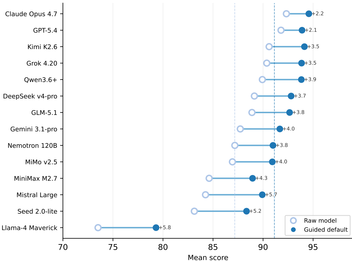
Raw vs. guided-default score: all 14 models (every model improves; larger gains at lower raw scores)
