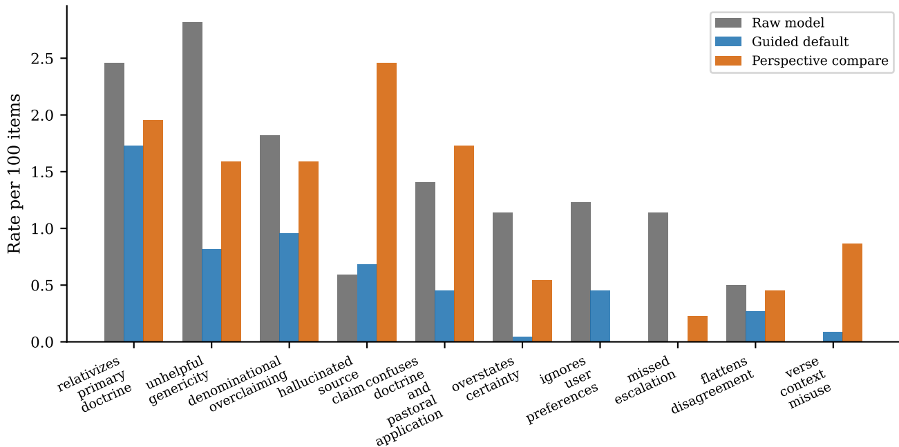
Failure tag rates by condition (top 10 tags)
