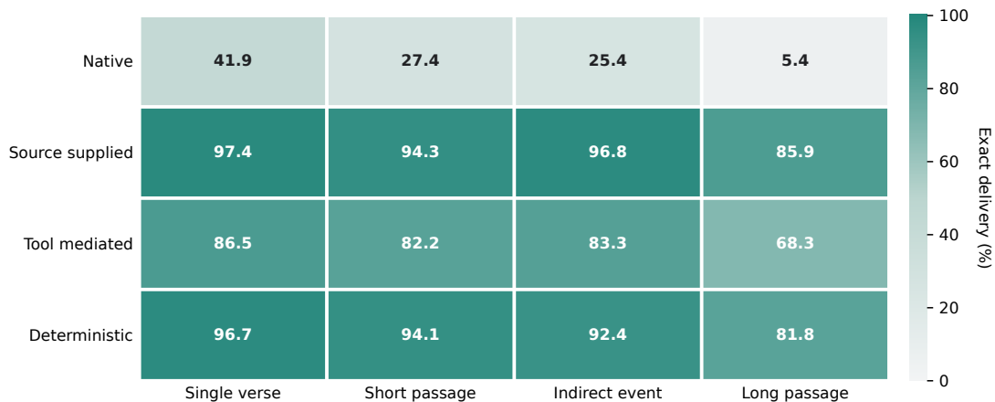
Figure 5: Exact delivery by passage stratum ( N = 540 per cell). “Indirect event” describes target construction; both prompt families were evaluated for every target.
