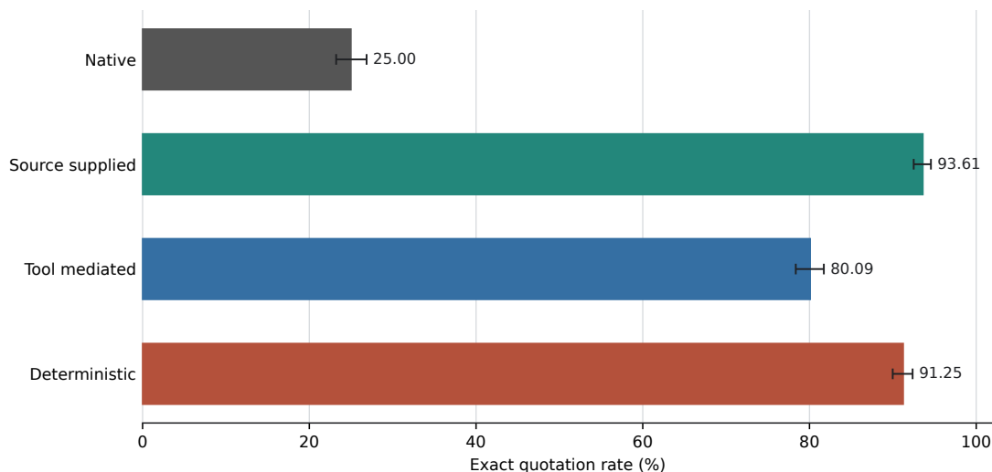
Figure 2: Exact delivery by condition with descriptive observation-level Wilson 95% intervals. All scheduled observations, including terminal provider errors, remain in the denominator.
