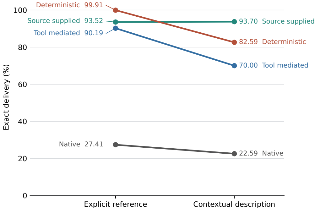
Figure 4: Exact delivery by caller prompt family ( N = 1,080 per cell). Contextual descriptions add a passage-identification burden, producing the largest declines in the tool-mediated and deterministic conditions.
