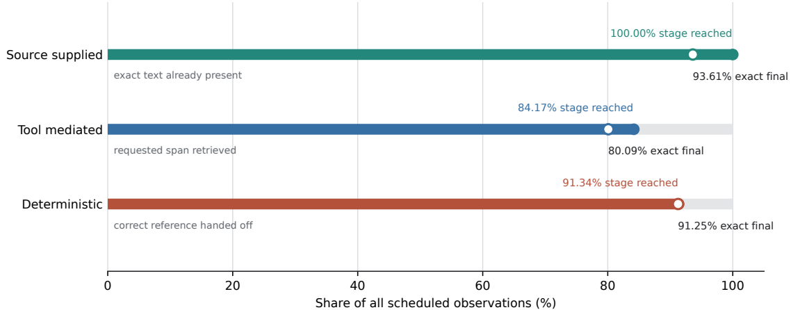
Figure 3: Failure moves to the stages that remain model-controlled. Filled markers show the share of all scheduled observations reaching the named source stage; open markers show path-adherent exact final delivery. The source-supplied condition begins at 100% because the exact span is given by construction.
