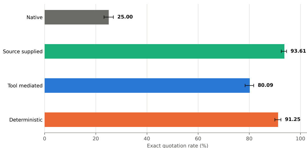
Figure 2: Exact delivery by condition with descriptive observation-level Wilson 95% intervals. All scheduled observations, including terminal provider errors, remain in the denominator.
