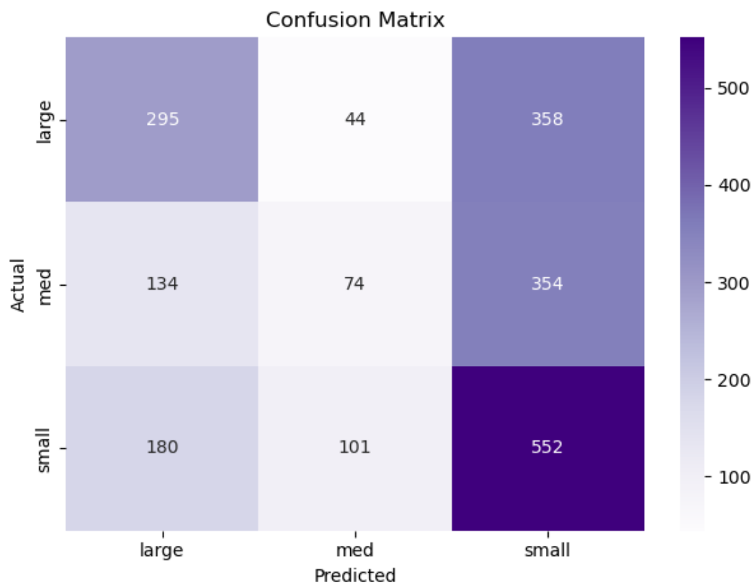
Figure 18: Confusion matrix for the Random Forest classifier.
