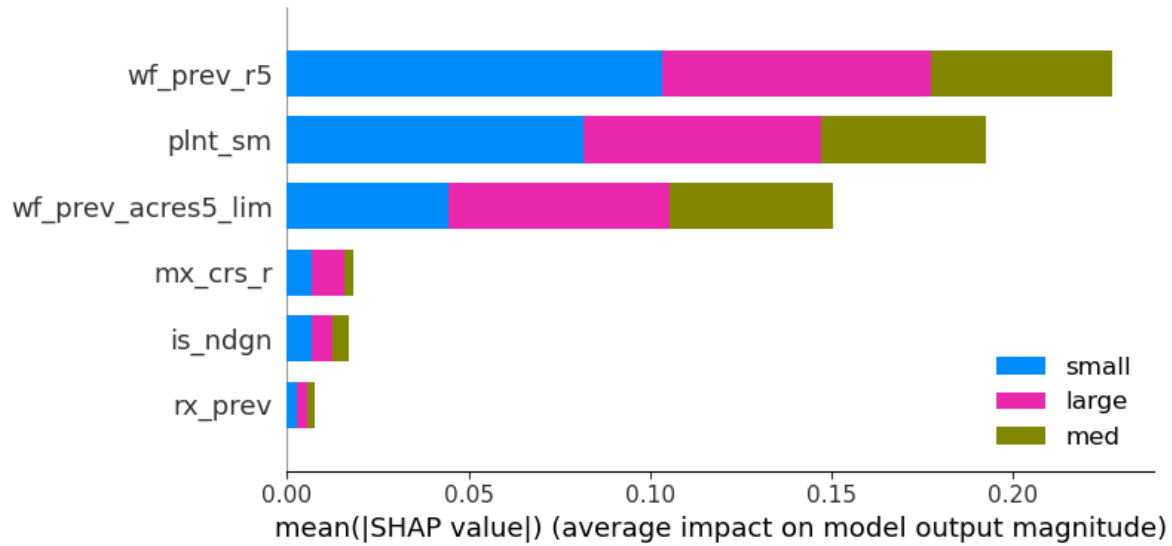
Figure 16: SHAP values for the Random Forest classifier.
