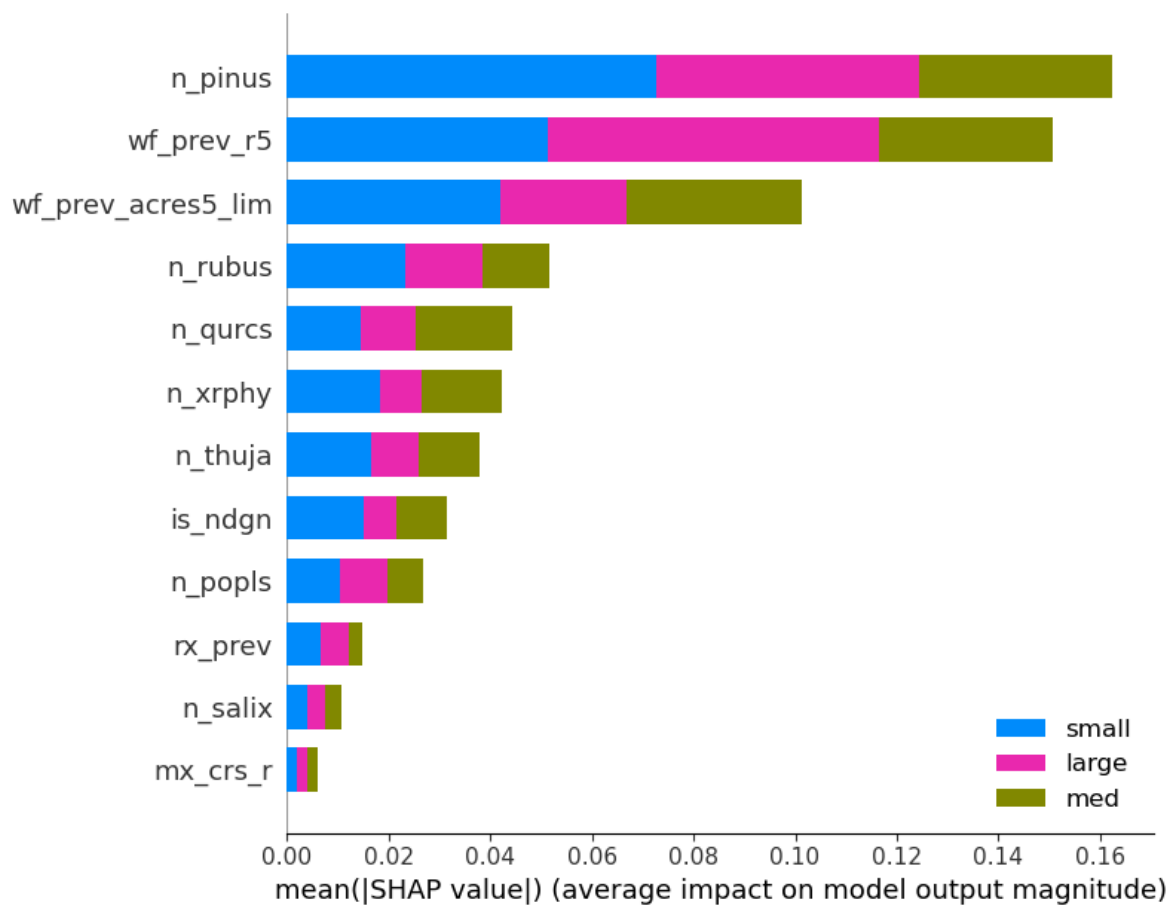
Figure 17: SHAP values for the Random Forest classifier with all plant species counts included separately.
