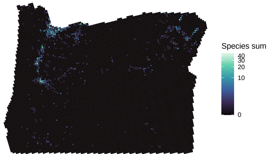
Black Cottonwood sums across Oregon
