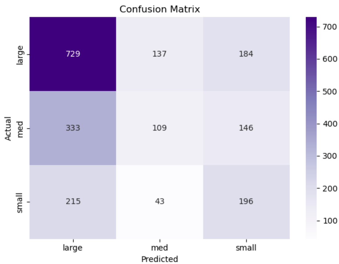
Figure 19: Confusion matrix for the Random Forest classifier with all plant species counts included separately.
