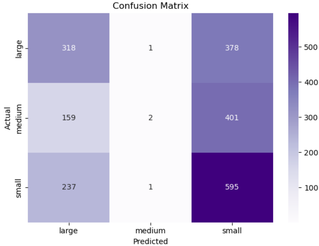
Figure 16: Confusion matrix for the Random Forest classifier.
