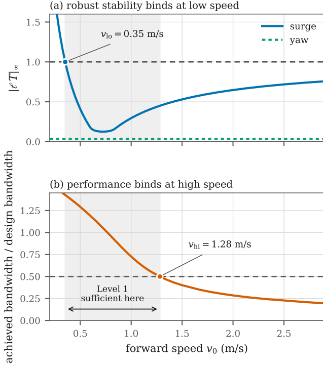
Fig. 2. Diagnostic 4. (a) Robust stability of the Level-1 compensator against the Level-2 linearization binds at low speed, where the quadratic-drag linearization is singular. (b) Achieved closed-loop bandwidth binds at high speed. The shaded band is the interval over which the Level-1 model supports the design. The yaw channel (a, dotted) never approaches the limit, so Level 2 changes nothing for yaw control.
