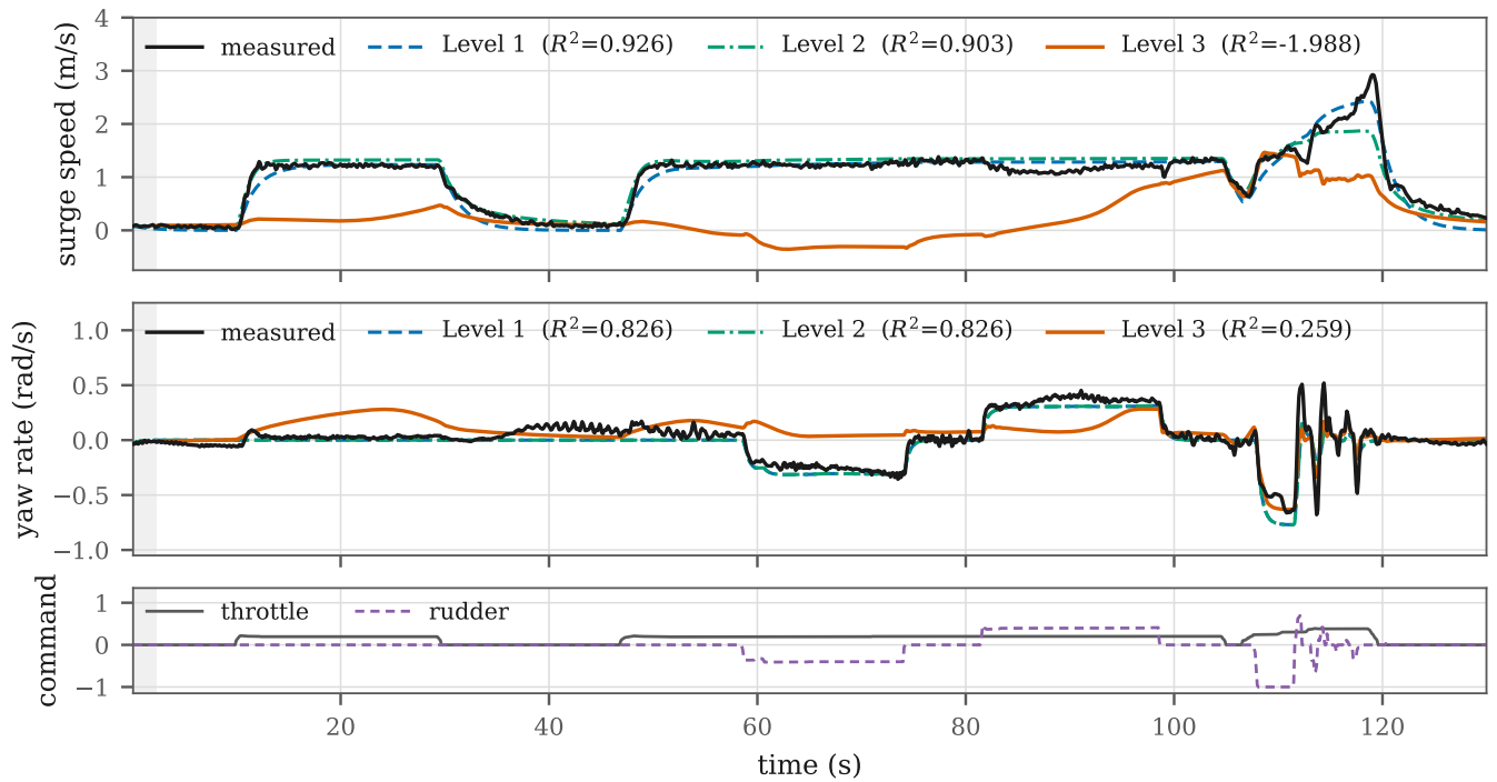
Fig. 6. All three levels under recursive simulation on the common 130 s trial. Levels 1 and 2 track the measured response; Level 3 diverges in surge, driving the predicted speed below zero for tens of seconds despite reaching the highest one-step accuracy of the three. Level 3 begins after 2 s of measured lag initialization, so it scores 1,279 rows against 1,300 for Levels 1 and 2.
