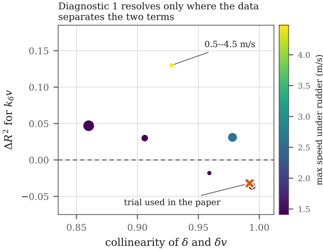
Fig. 3. Diagnostic 1 repeated on each manual-mode record of the supplementary corpus. The horizontal axis is the correlation between \delta and \delta v over the samples with rudder applied, so records to the right cannot separate a constant gain from a speed-scaled one. Marker area is record length and colour is the highest speed reached under rudder. The cross marks the identification trial used throughout the paper.
