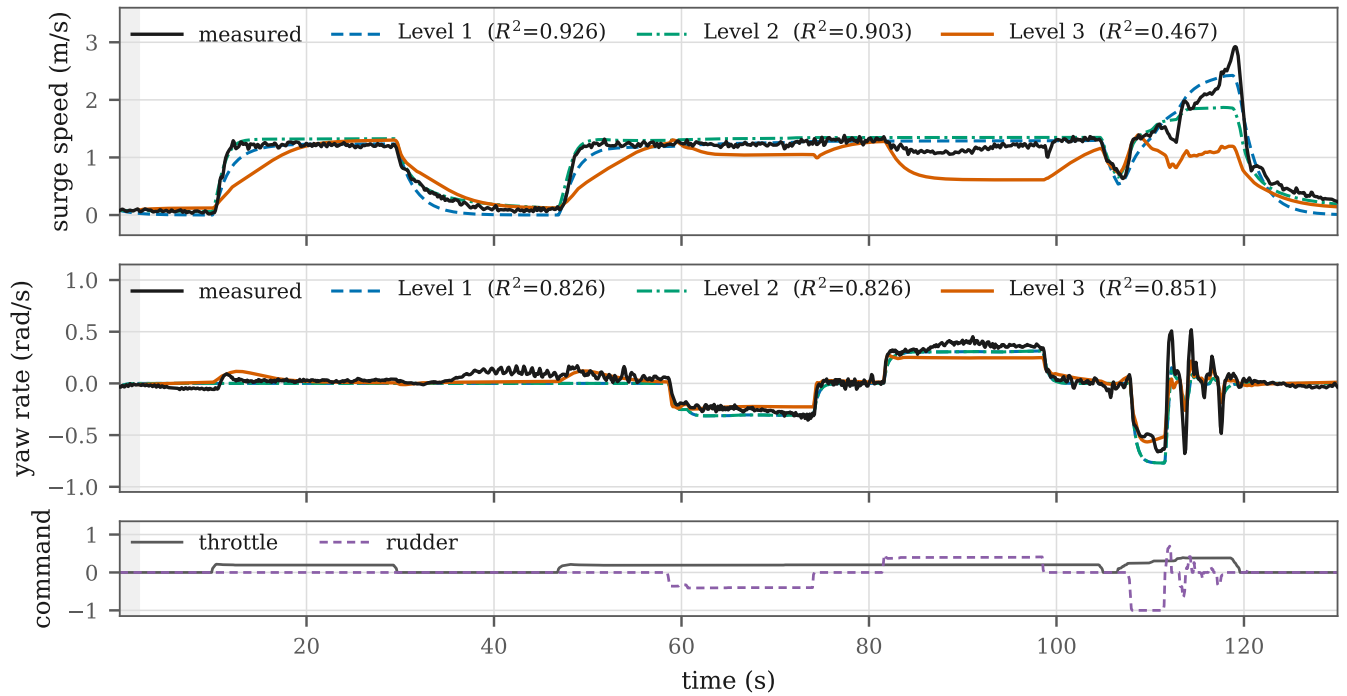
captionAll three levels simulated on the common 130 s trial, with Level 3 trained on the curated logs. Level 3 begins after 2 s of measured lag initialization, so it scores 1,279 rows against 1,300 for Levels 1 and 2, and all three are scored on those same rows.
