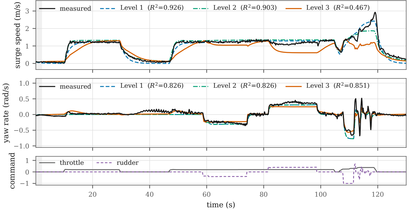
Fig. 5. All three levels simulated on the common 130 s trial. Level 3 begins after 2 s of measured lag initialization, so it scores 1,279 rows against 1,300 for Levels 1 and 2, and all three are scored on those same rows.
