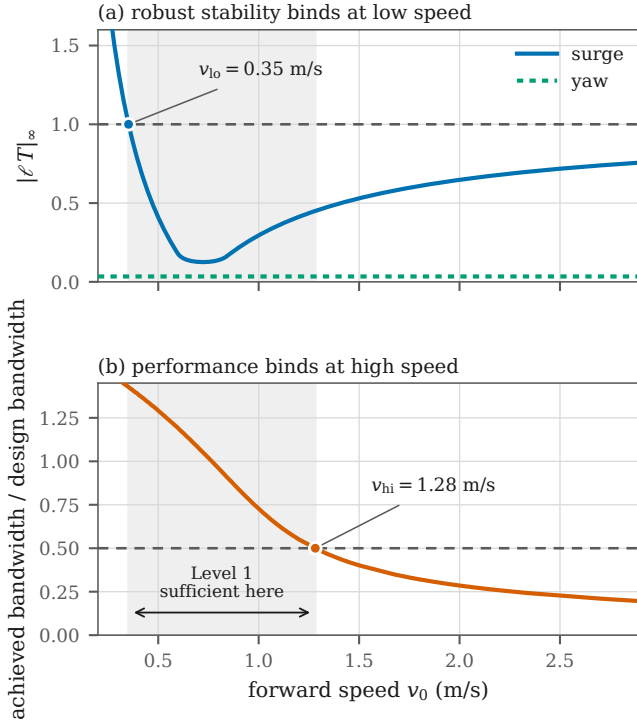
Fig. 3. Diagnostic 4. (a) Robust stability of the Level-1 compensator against the Level-2 linearization binds at low speed, where the quadratic-drag linearization is singular. (b) Achieved closed-loop bandwidth binds at high speed. The shaded band is the interval over which the Level-1 model supports the design. The yaw channel (a, dotted) never approaches the limit.
