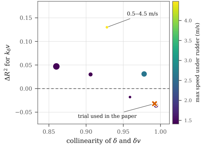
Fig. 4. Diagnostic 1 repeated on each manual-mode record of the supplementary set. The horizontal axis is the correlation between \delta and \delta v over the samples with rudder applied, so records to the right cannot separate a constant gain from a speed-scaled one. Marker area is record length and colour is the highest speed reached under rudder. The cross marks the identification trial used throughout the paper.
