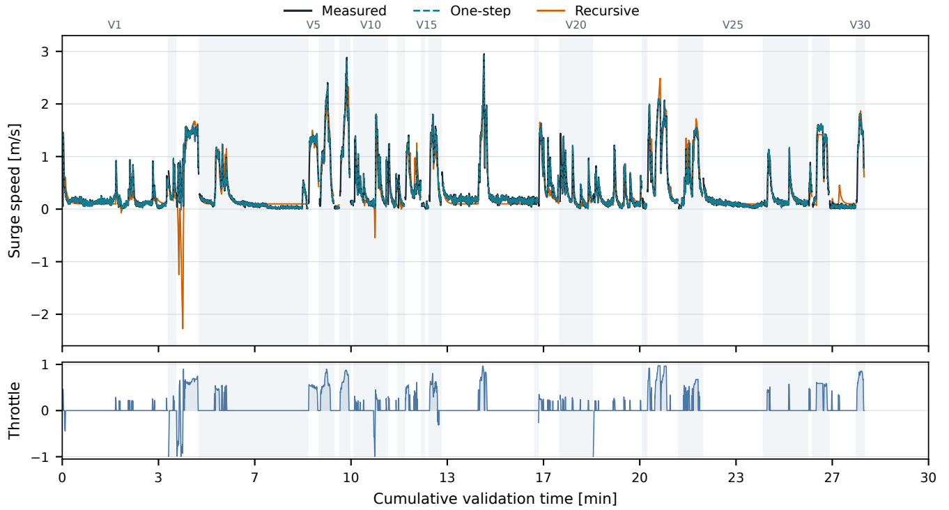
Fig. 3. Level 3 surge prediction on the complete slow-region validation set of 30 segments from 28 held-out source logs. Each segment is initialized with 2 s of measured history. One-step prediction continues to use measured state history; recursive simulation feeds predicted states back while replaying recorded throttle. Alternating backgrounds and short gaps mark segment boundaries. Reported NRMSE values are segment-macro averages over speed and yaw-rate errors normalized by training-only channel scales.
