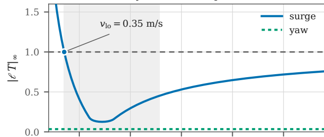
(a) robust stability binds at low speed
