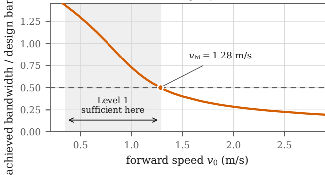
(b) performance binds at high speed
