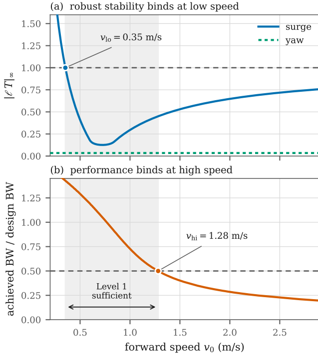
Fig. 1. Diagnostic 4. (a) Robust stability of the Level-1 compensator against the Level-2 linearization binds at low speed, where the quadratic-drag linearization is singular. (b) Achieved closed-loop bandwidth binds at high speed. The shaded band is the interval over which the Level-1 model supports the design. The yaw channel (a, dotted) never approaches the limit, so Level 2 changes nothing for yaw control.
