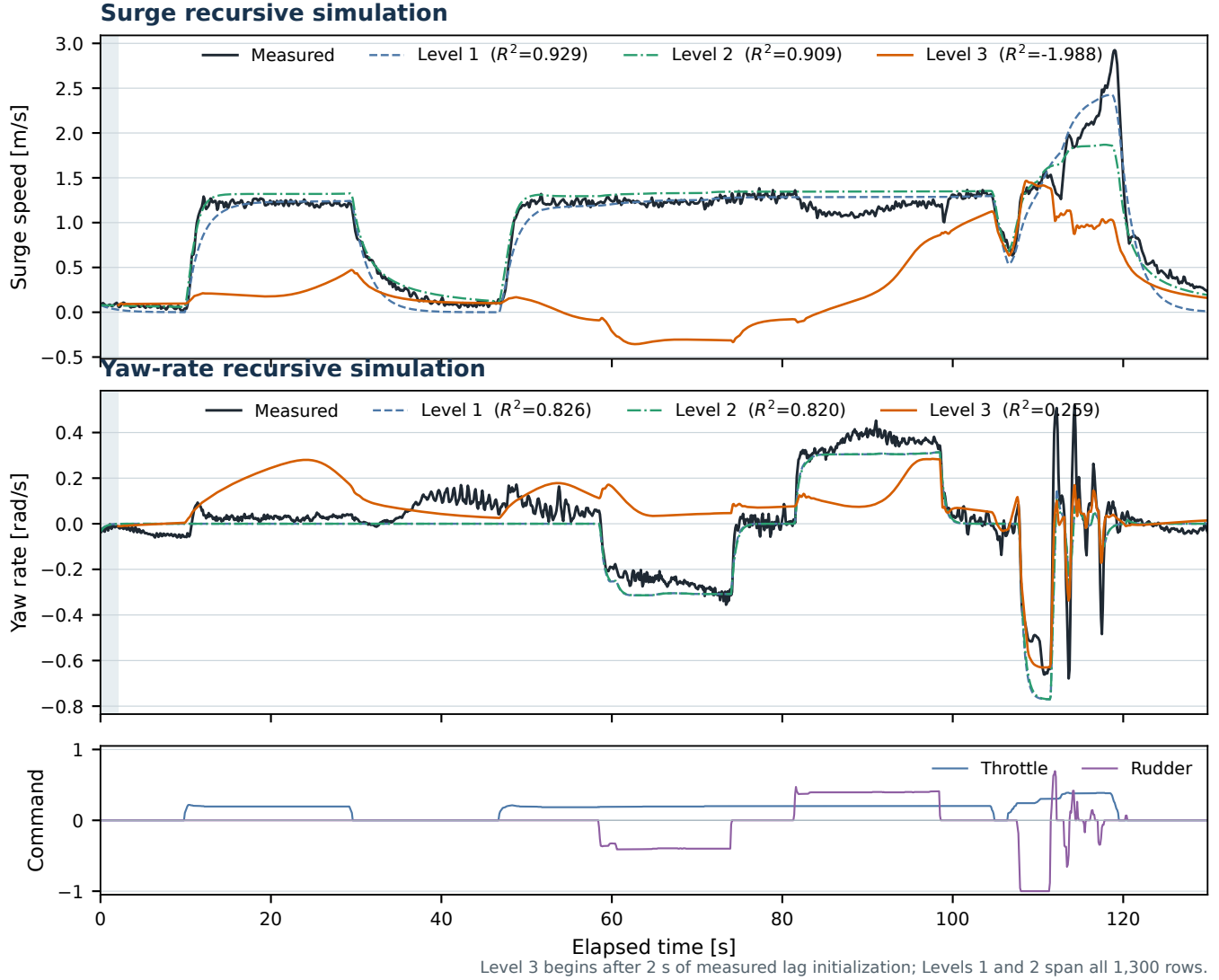
Fig. 3. All three levels under recursive simulation on the common 130 s trial. Levels 1 and 2 track the measured response; Level 3 diverges in surge, driving the predicted speed below zero for tens of seconds despite reaching the highest one-step accuracy of the three. Level 3 begins after 2 s of measured lag initialization, so it scores 1,279 rows against 1,300 for Levels 1 and 2.
