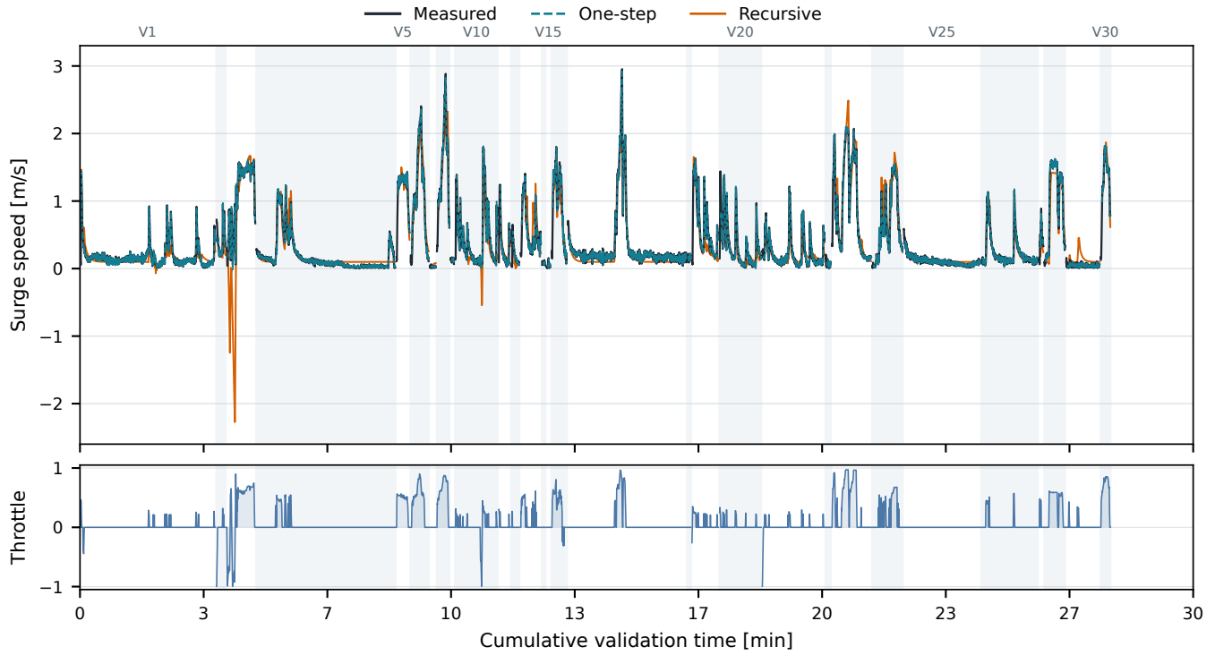
Fig. 2. Level 3 surge prediction on the complete slow-region validation set of 30 segments from 28 held-out source logs. Each segment is initialized with 2 s of measured history. One-step prediction continues to use measured state history; recursive simulation feeds predicted states back while replaying recorded throttle. Alternating backgrounds and short gaps mark segment boundaries. Reported NRMSE values are segment-macro averages over speed and yaw-rate errors normalized by training-only channel scales.
