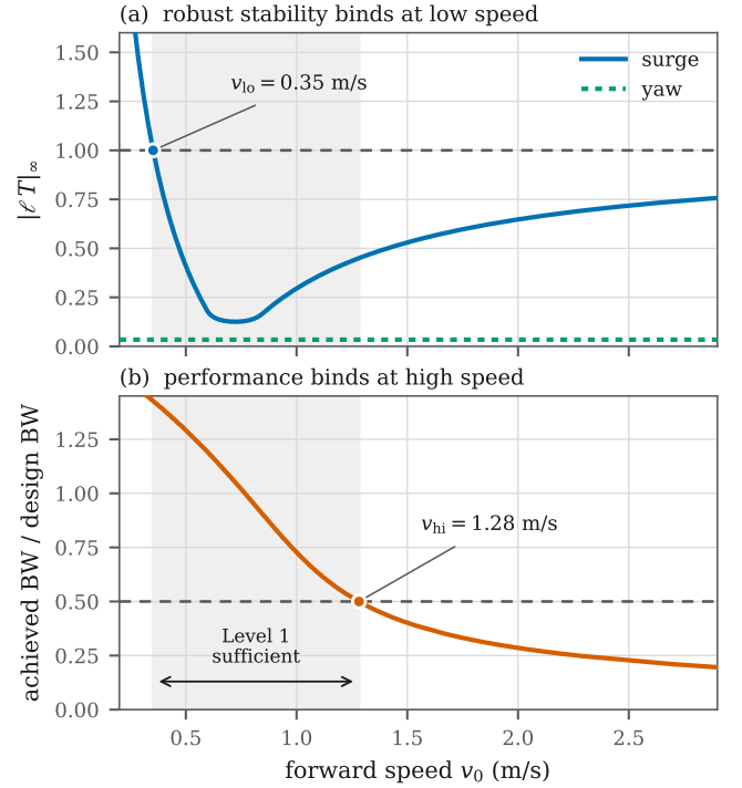
Fig. 1. Diagnostic 4. (a) Robust stability of the Level-1 compensator against the Level-2 linearization binds at low speed, where the quadratic-drag linearization is singular. (b) Achieved closed-loop bandwidth binds at high speed. The shaded band is the interval over which the Level-1 model supports the design. The yaw channel (a, dotted) never approaches the limit, so Level 2 changes nothing for yaw control.
