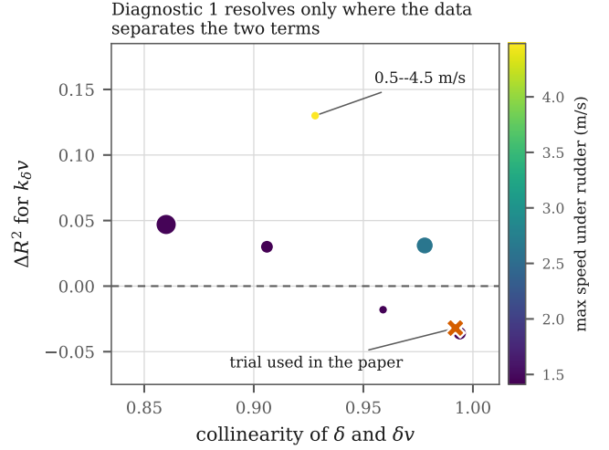
Fig. 3. Diagnostic 1 repeated on each manual-mode record of the supplementary corpus. The horizontal axis is the correlation between \delta and \delta v over the samples with rudder applied, so records to the right cannot separate a constant gain from a speed-scaled one. Marker area is record length and colour is the highest speed reached under rudder. The cross marks the identification trial used throughout the paper.
