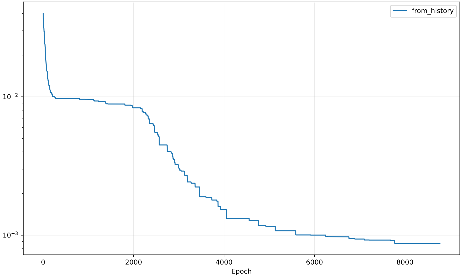
Running best validation loss
