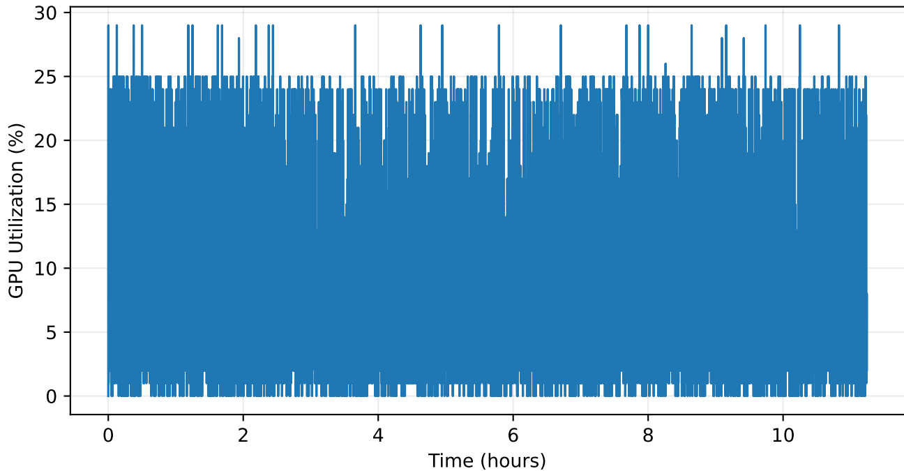
GPU Utilization
