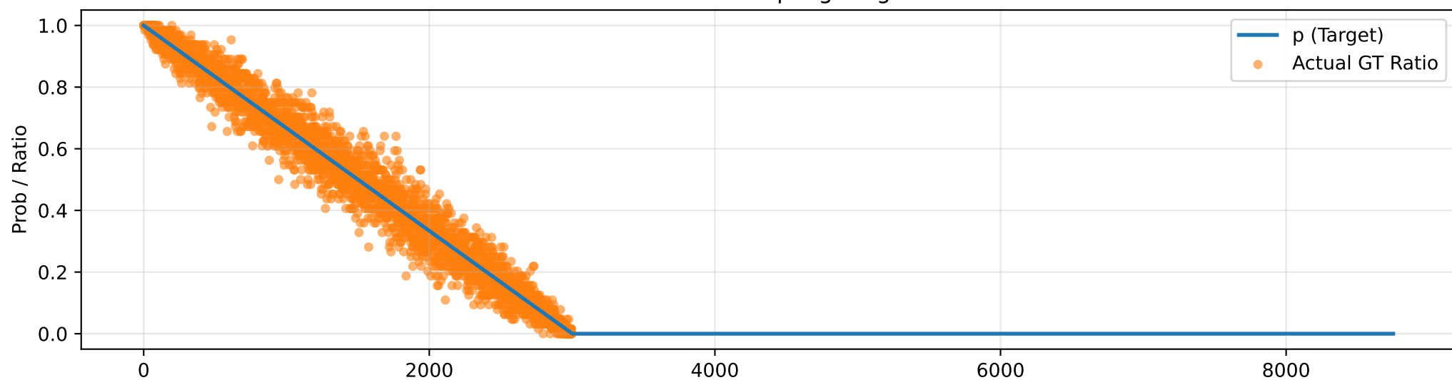
Scheduled Sampling Progress
