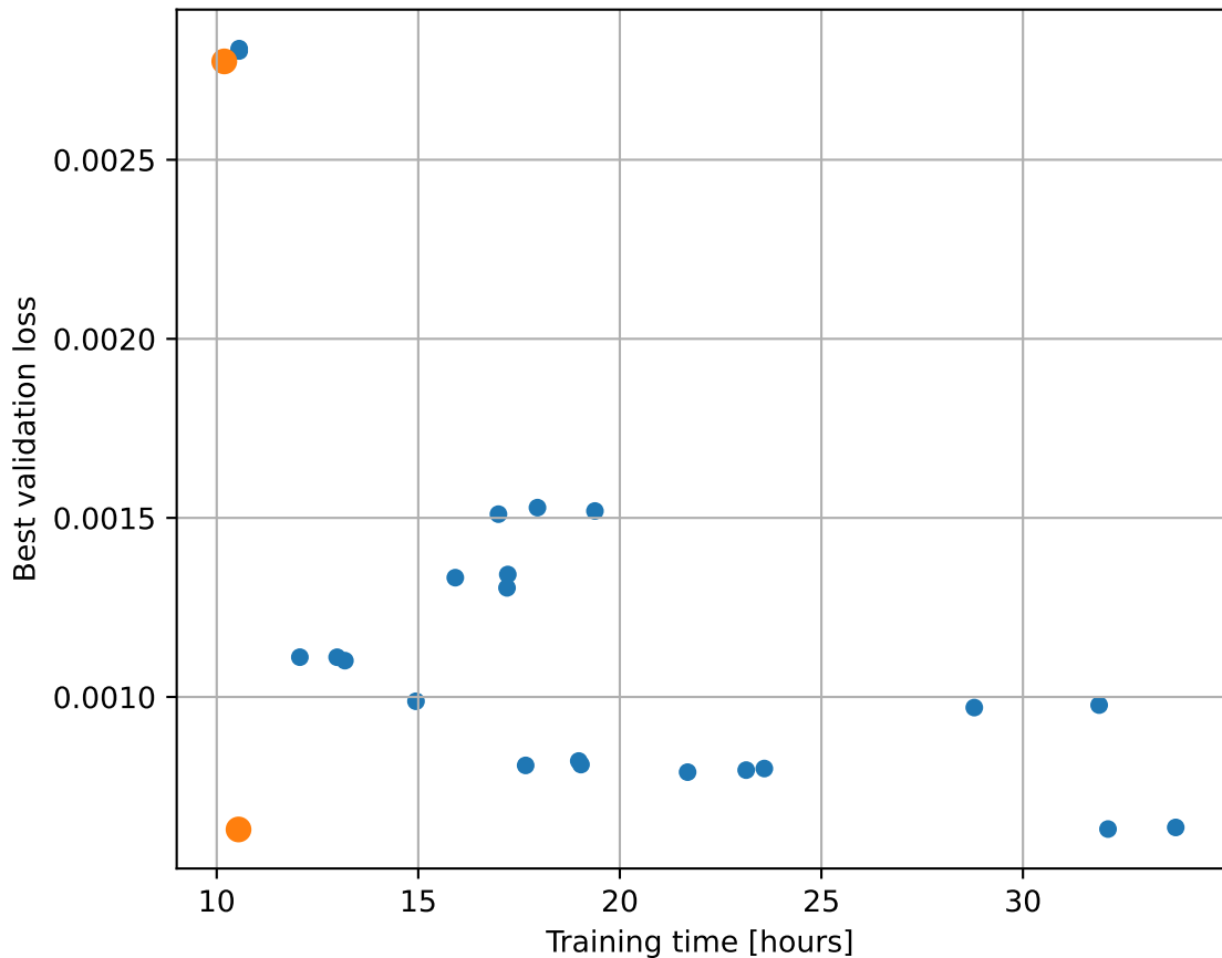
Pareto front: minimize (loss, time)
