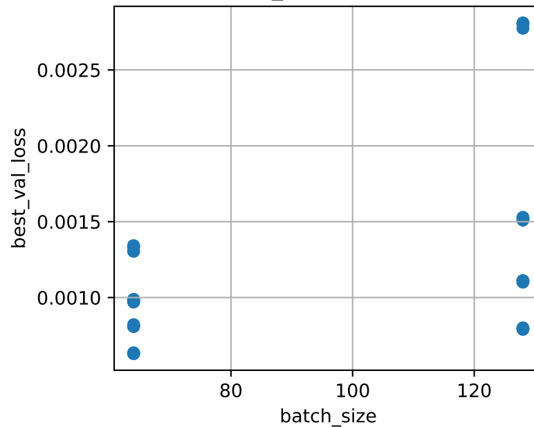
batch_size vs val loss
