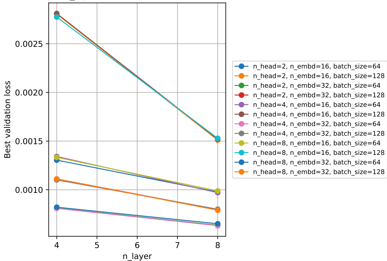
Effect of n_layer on validation loss (others fixed)
