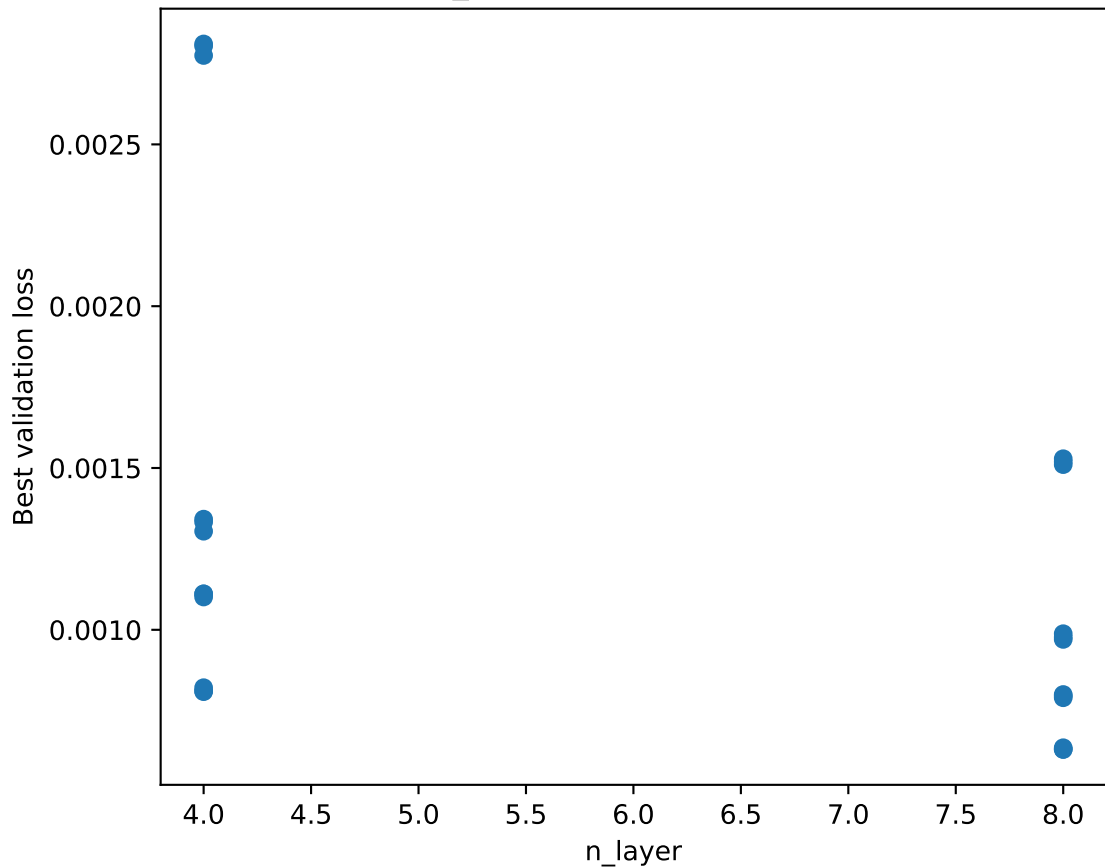
n_layer vs validation loss
