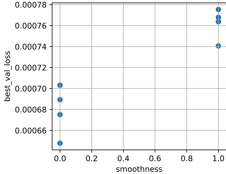
smoothness vs val loss
