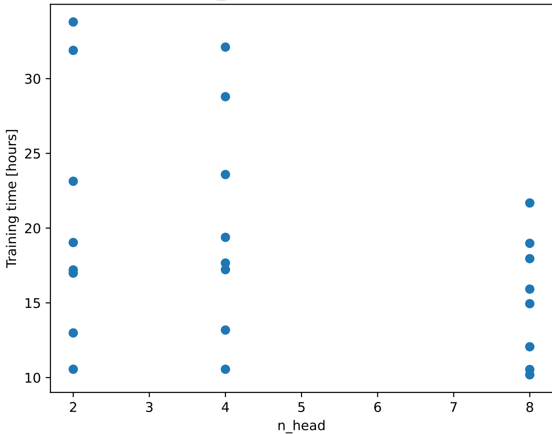
n_head vs training time
