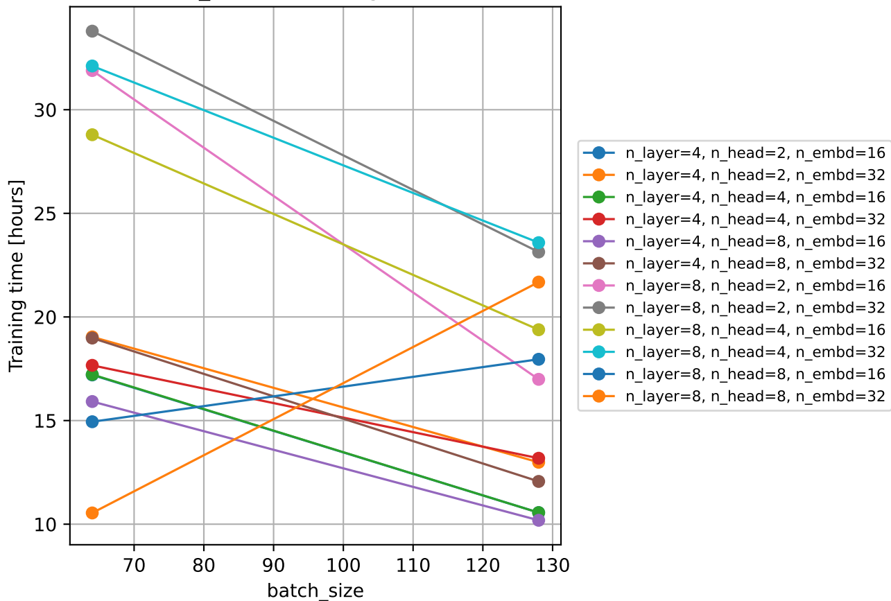
Effect of batch_size on training time (others fixed)
