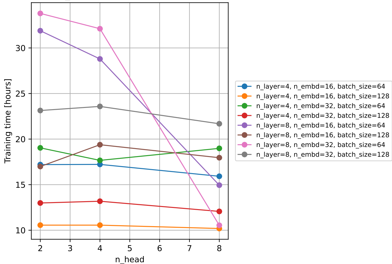
Effect of n_head on training time (others fixed)
