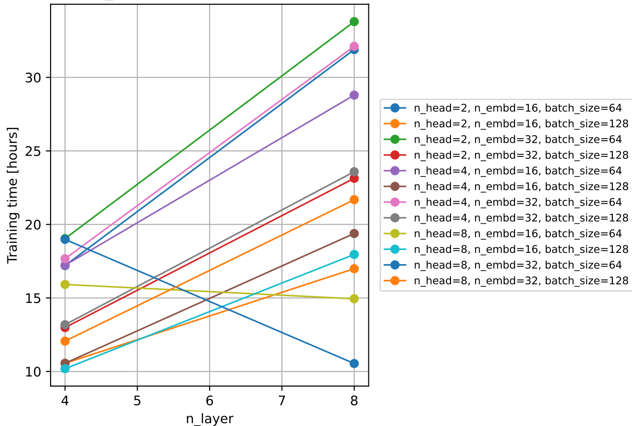
Effect of n_layer on training time (others fixed)
