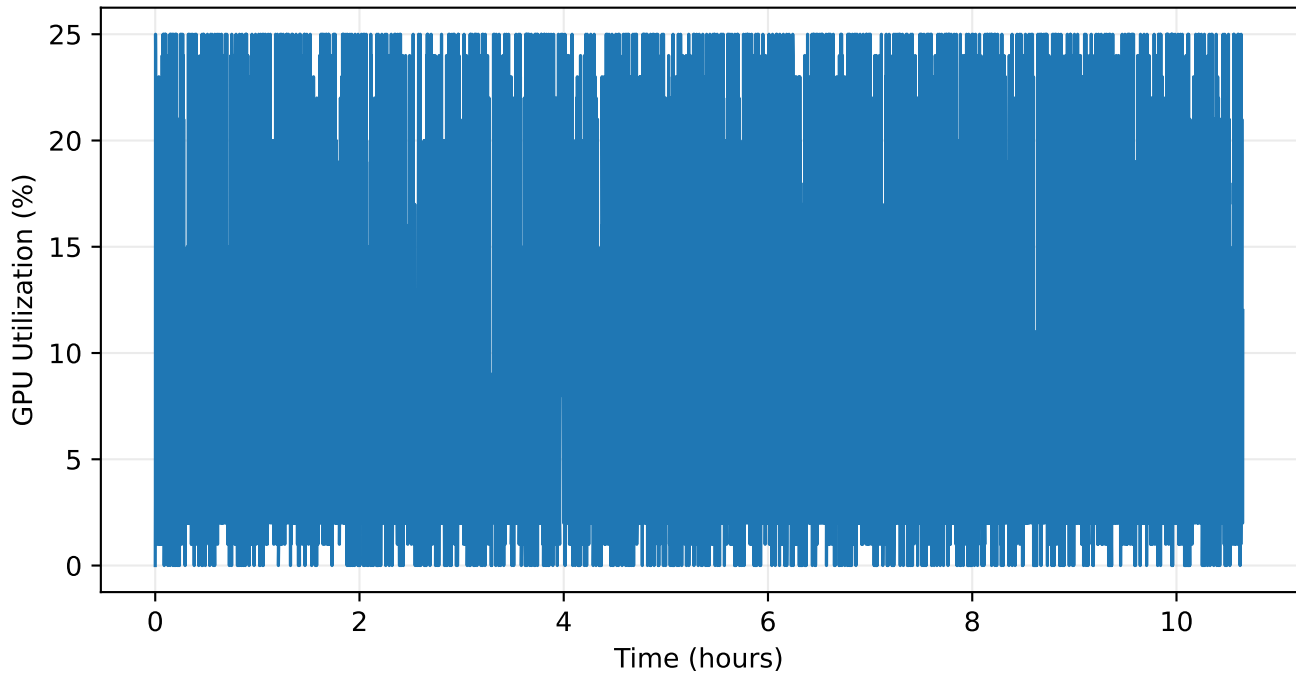
GPU Utilization
