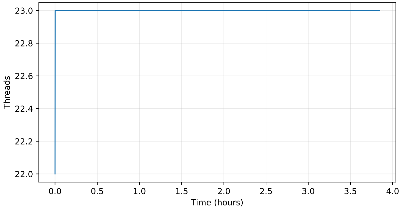
Process Threads
