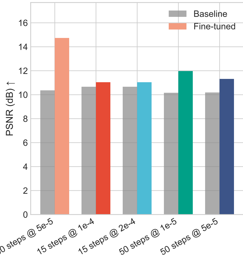
PSNR Comparison
