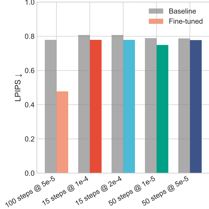
LPIPS Comparison (Lower is Better)
