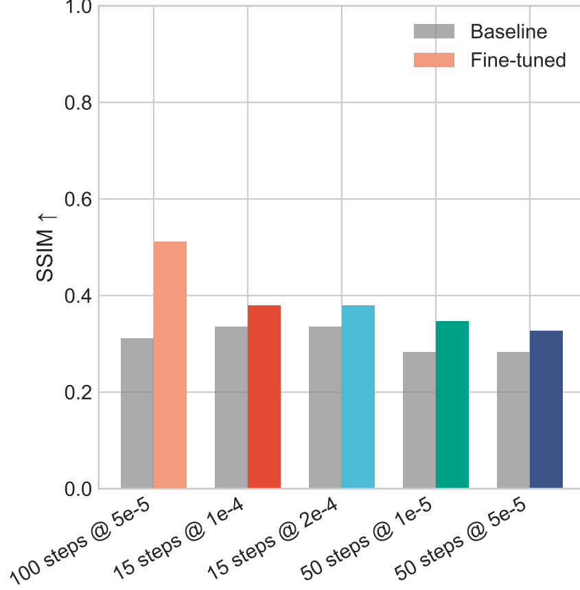
SSIM Comparison
