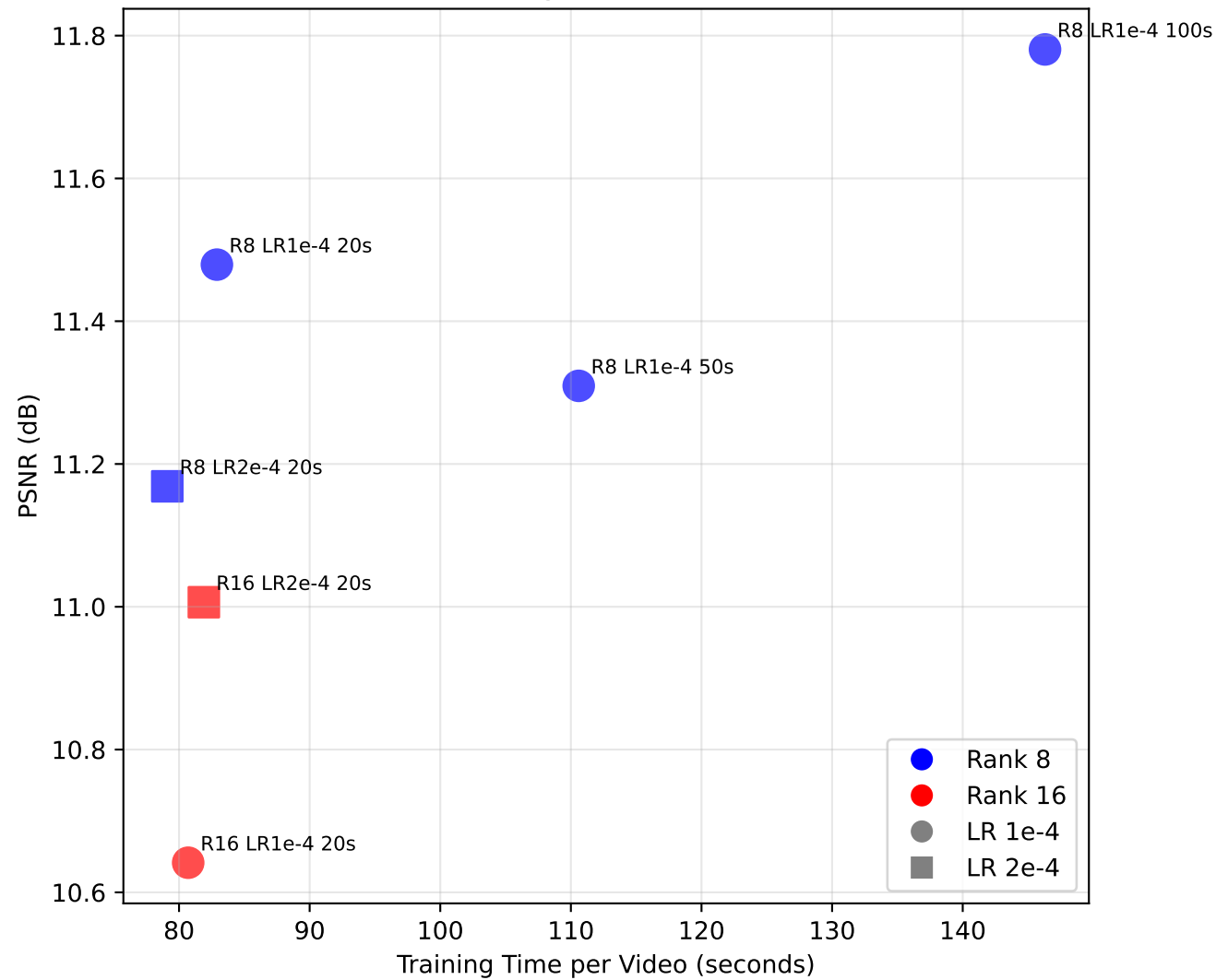
Training Time vs PSNR
