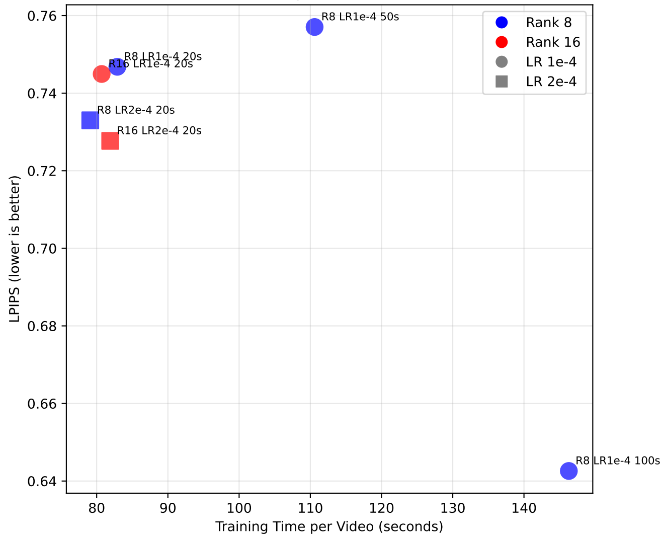
Training Time vs LPIPS
