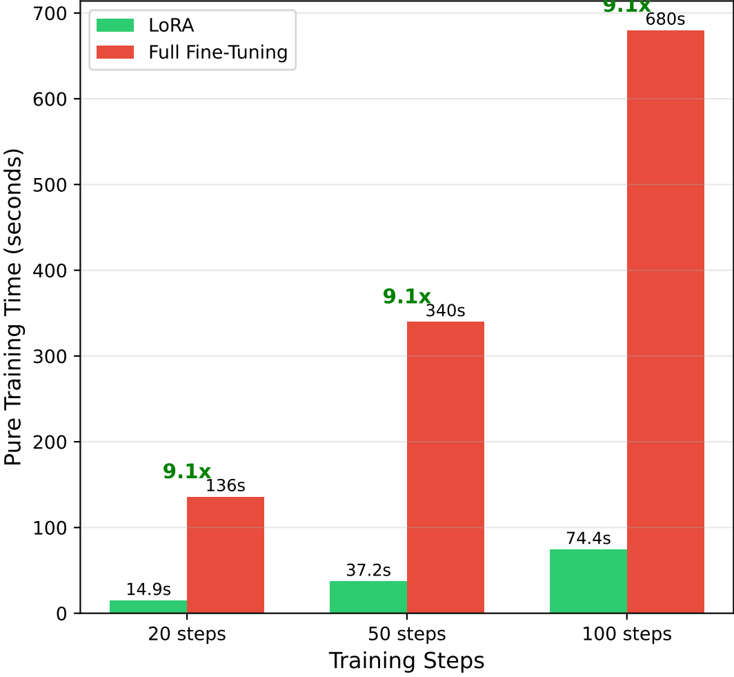
Pure Training Time Comparison (Gradient Steps Only - No Overhead)
