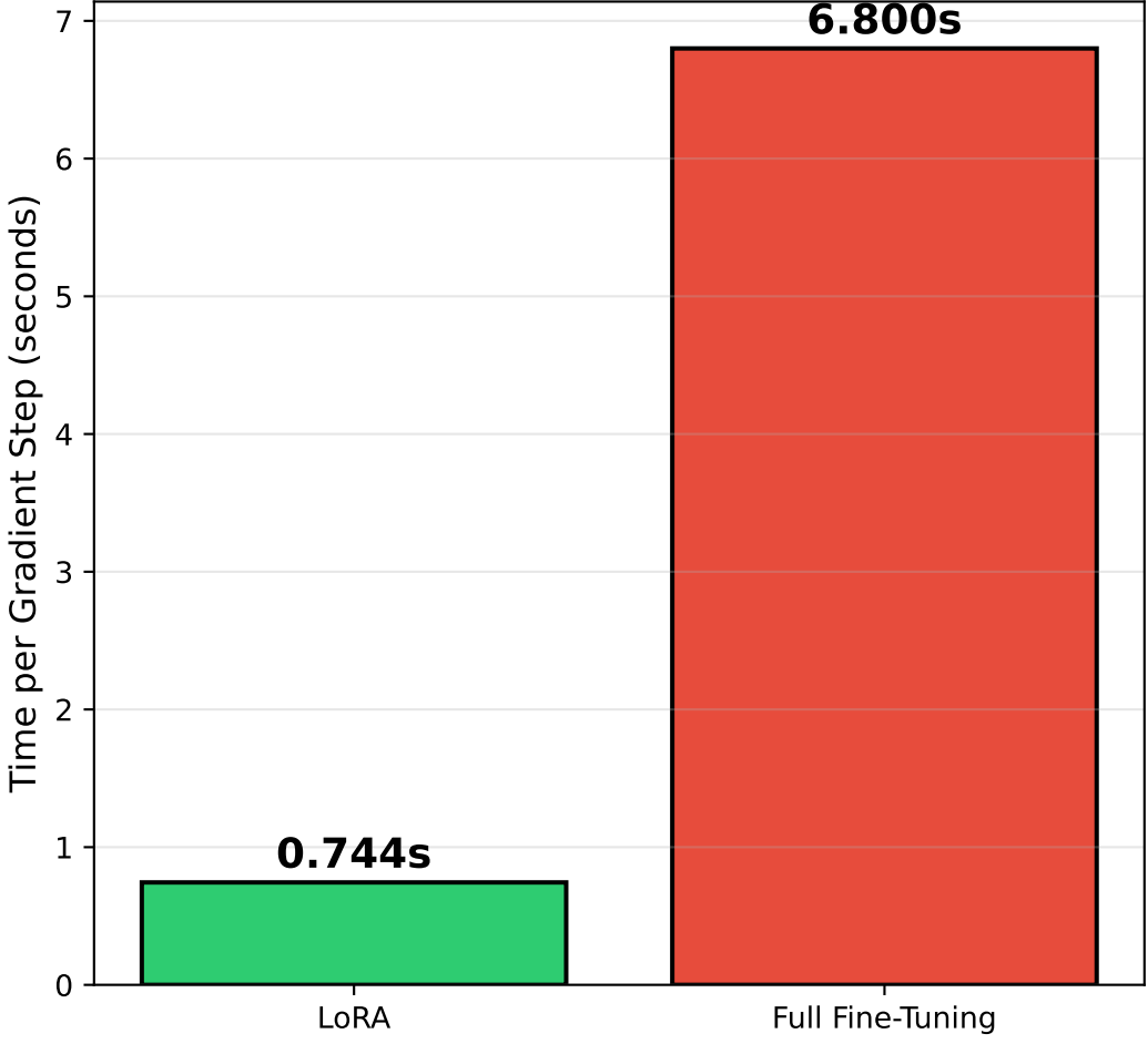
Time per Gradient Step
