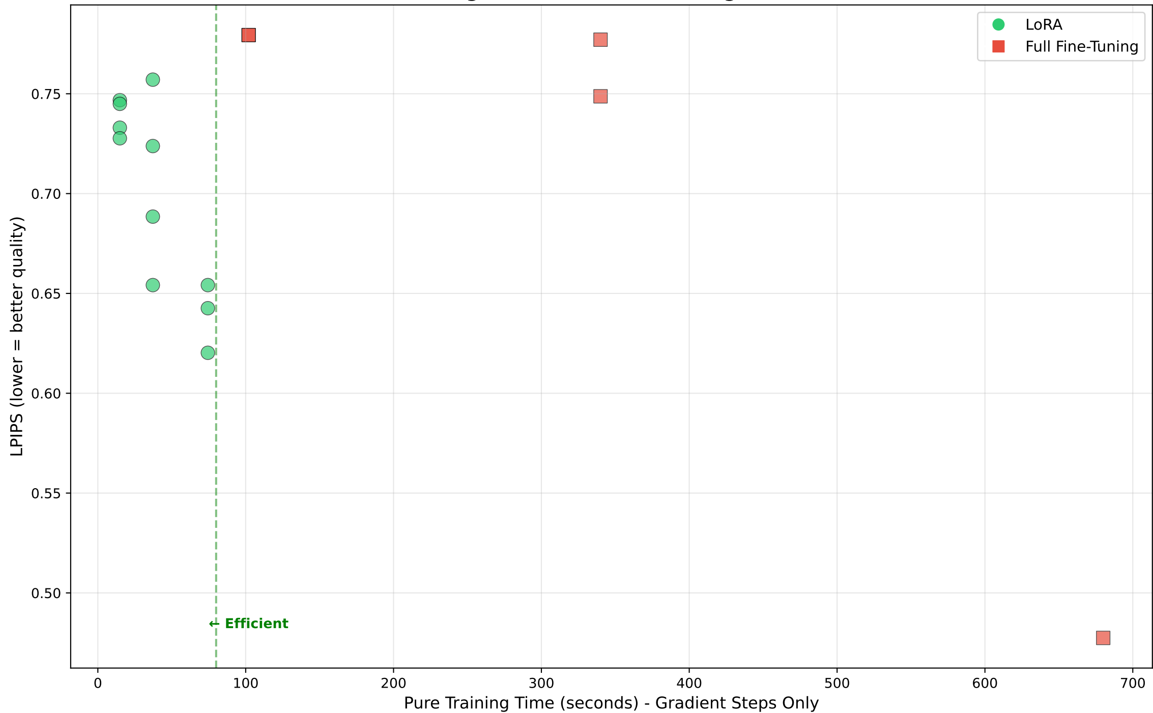
Pure Training Time vs Quality (Excluding Model Load & Encoding Overhead)
