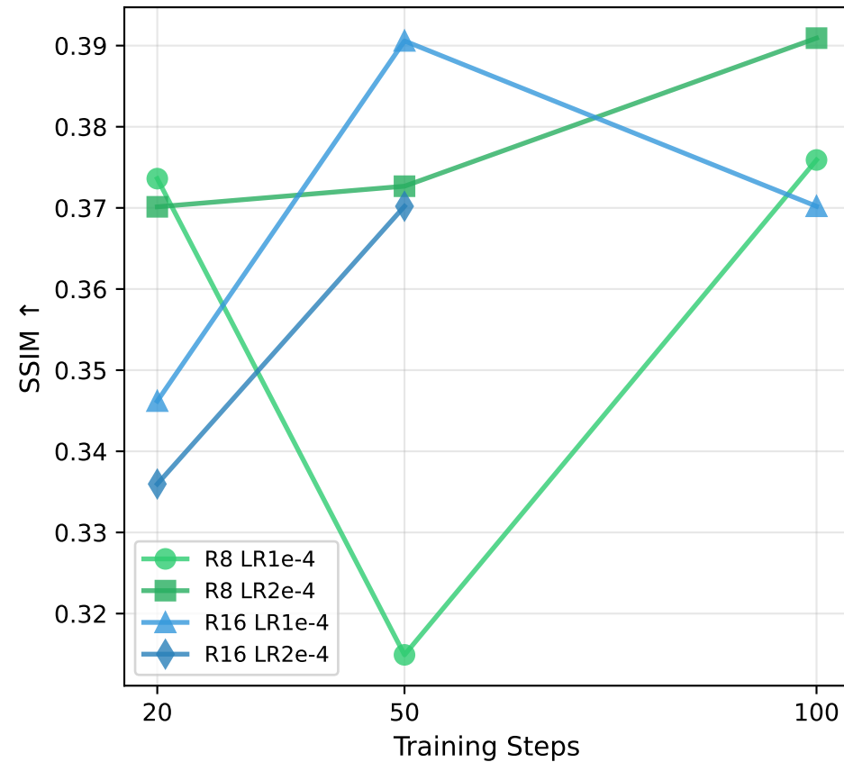
LoRA Performance vs Training Steps
