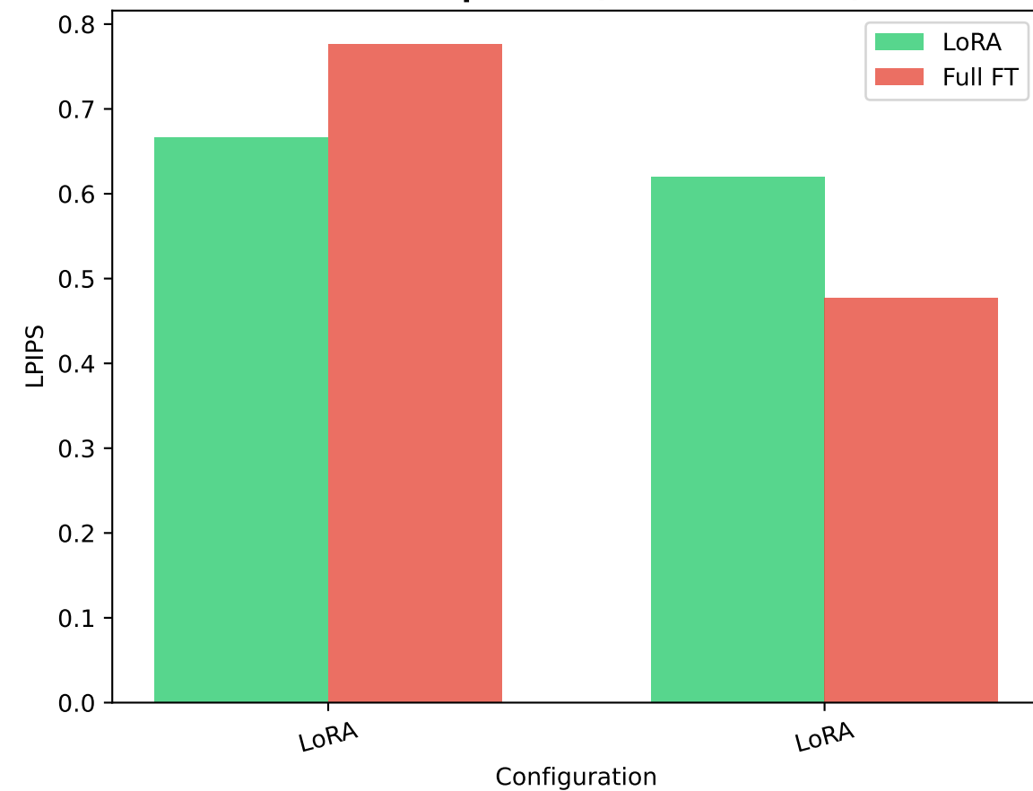
LPIPS Comparison (Lower = Better)
