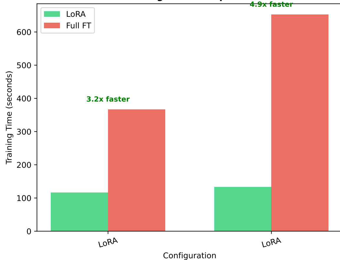
Training Time Comparison
