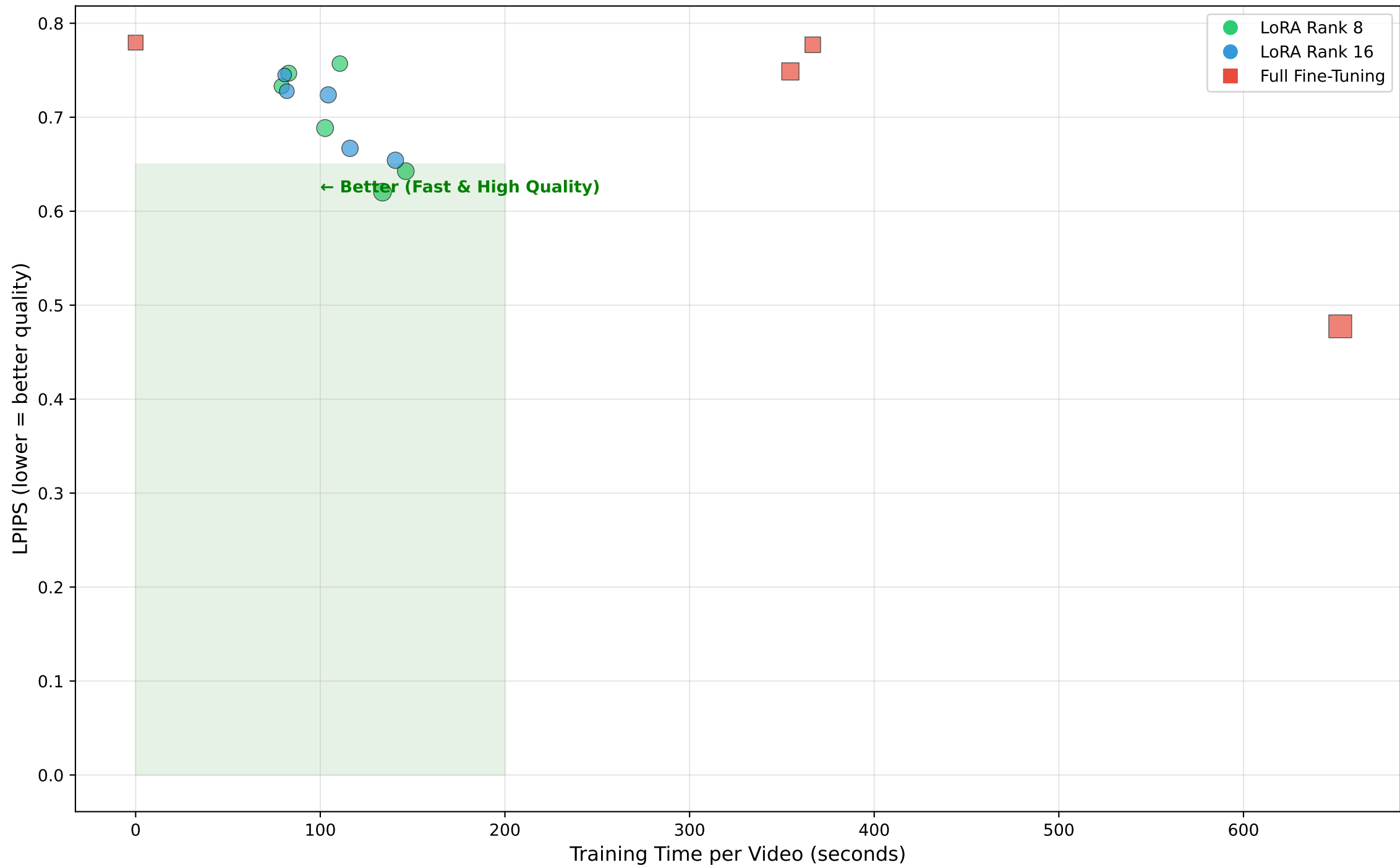
Efficiency Overview: All Methods (Bubble size = PSNR)
